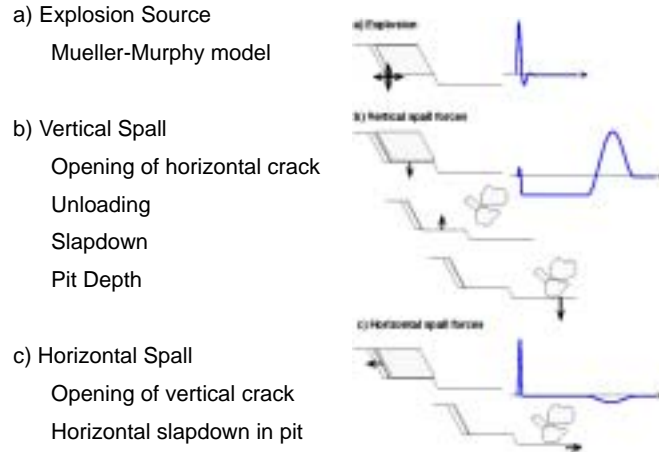
Figure 4: The three components of the equivalent mining explosion source model are represented pictorially. They consist of (a) the directly coupled energy from the contained explosion modeled as a Mueller-Murphy source function, (b) vertical spall due to the tensile failure of near-surface materials and (c) horizontal spall accompanying cast blasting when overburden is cast horizontally into a pit.
