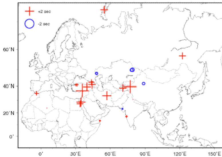
CUB Cluster Origin Time Offsets
