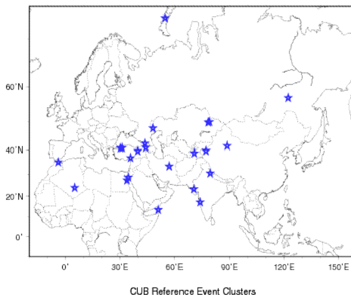
Figure 1. Locations of the explosion and earthquake clusters studied indicated by stars.
