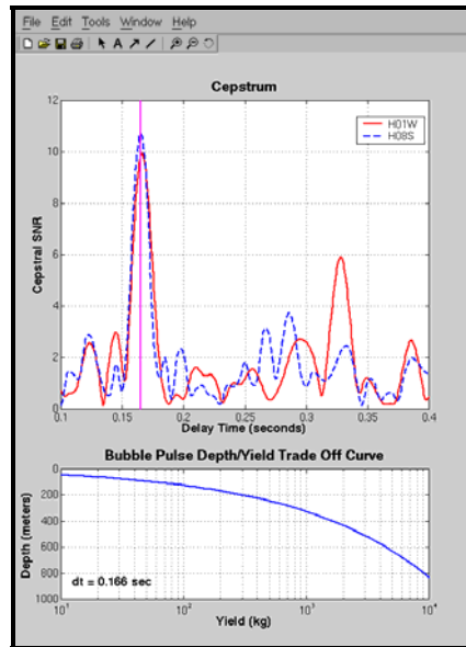
Figure 8. Example of a Cepstral Analysis Tool. The ability to review and modify cepstral results will be a new feature of this ACD. This tool allows the analyst to confirm the very important event characterization measurement. The estimated delay time (the first peak in the cepstrum) determines a depth/yield trade-off curve that will be used in determining a hydroacoustic magnitude. The automatic system picks the maximum peak that sometimes corresponds to the second bubble pulse and needs to be corrected by the analyst. The cepstra can also provide strong evidence for phase association as shown in this example with two signals measured at widely separated hydrophones that have nearly identical cepstral peaks.
