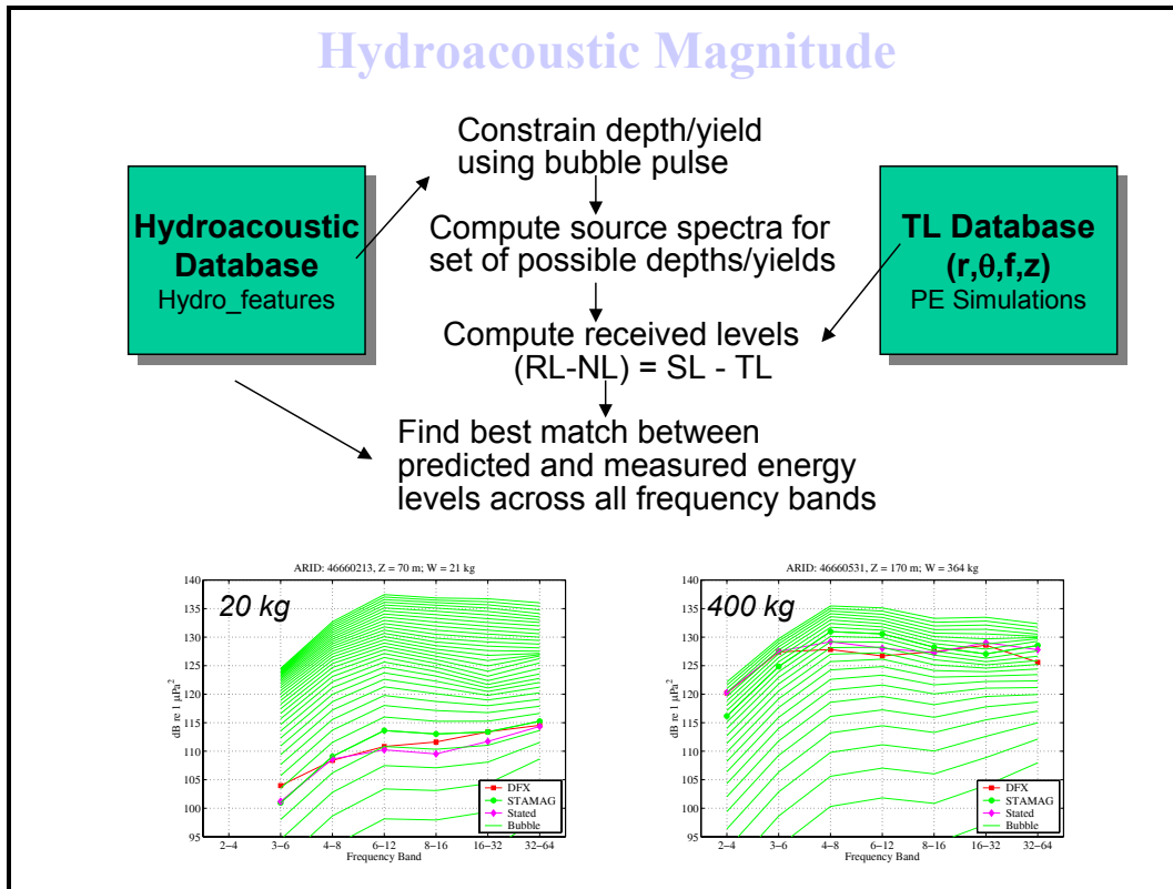
Figure 9. Estimation of hydroacoustic magnitudes. The received signal levels are matched to simulations based on source path and constrained using the bubble pulse depth/yield trade-off. The two examples use the actual measurements from explosions with nominal yields of 20-kg and 400-kg TNT equivalent.
