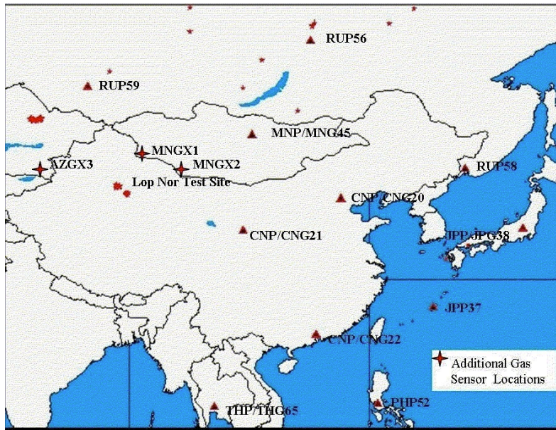
Figure 8. Recommended additional sensors to enhance detection capability of IMS network for Lop Nor.
