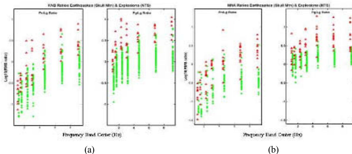
Figure 6. Scatter plots of Pn/Lg and Pg/Lg ratios for Skull Mountain earthquakes and NTS nuclear explosions at stations Kanab, Utah, (KNB) (a) and Mina, Nevada, (MNA) (b).
