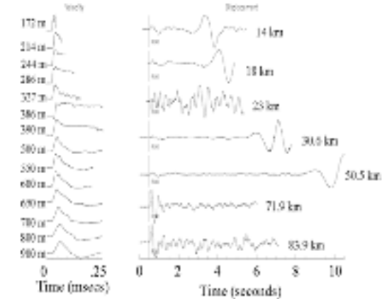
Figure 3. Near-field (left) and near regional seismic (right) waveforms from the 1987/07/17 event.
