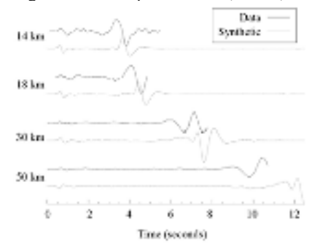
Figure 4. Synthetic and observed seismograms for the 1987/07/17 event. Synthetics were created using wavenumber integration and were low pass filtered at 2 Hz.
