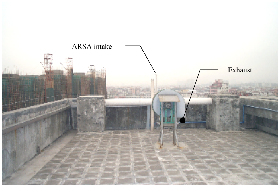
Figure 2. ARSA intake and fume hood vent location
