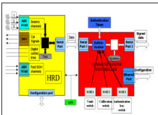
Figure 7. Internal data flow of the new digitizer.
