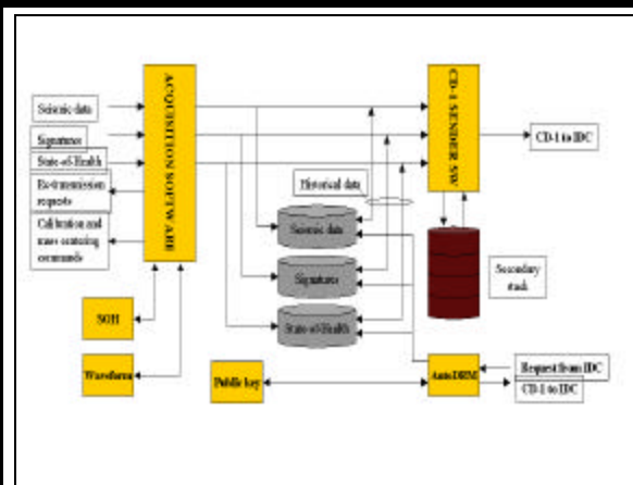
Figure 10. Data flow diagram of NAQSServer.
