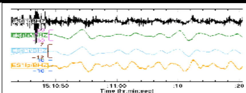
Figure 17. Background noise under new configuration, ES01i=Integrated data, ES1p=LP at 1Hz
