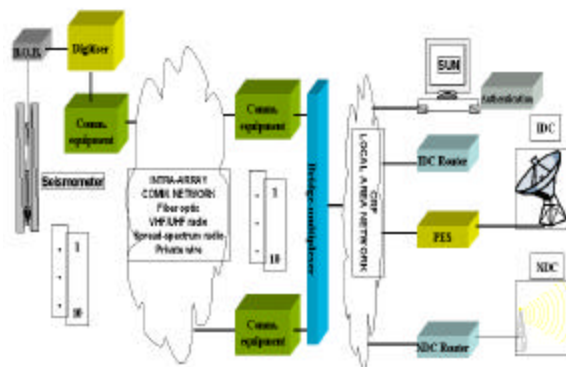
Figure 9. Block diagram of major components of the array.
