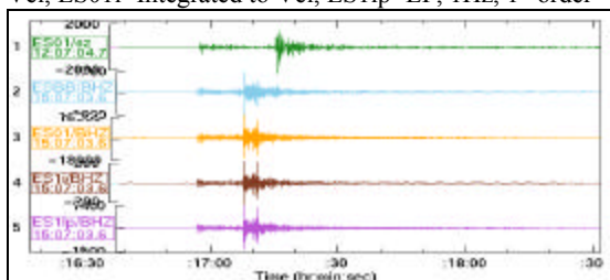
18A. Raw data, ES1lp is LP at 1.0 Hz
