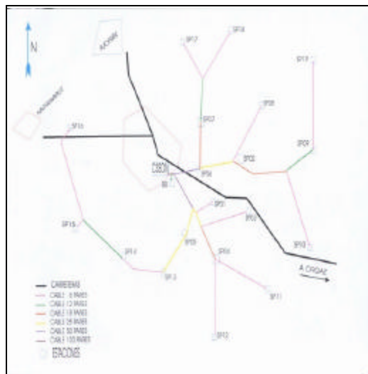
Figure 3, Power and Communications Distribution Network.
