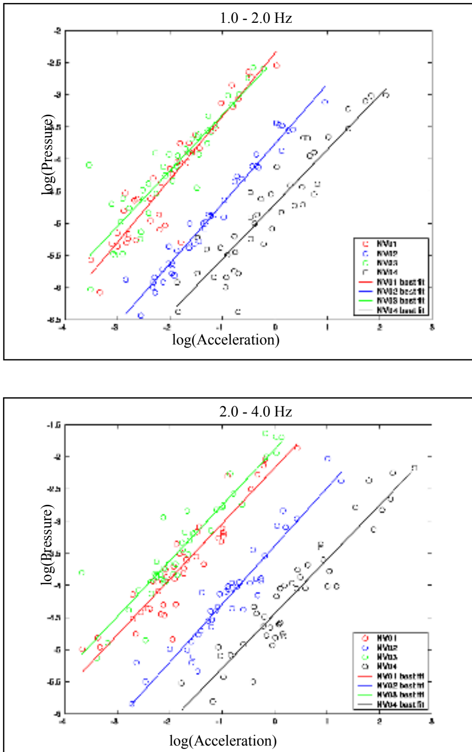
Figure 6. RMS Pressure versus RMS Acceleration for seismo-acoustic events. The data below 1 Hertz is contaminated by noise, and above 4 Hertz the response of the infrasound sensor hoses can further bias the measurements. The difference between NV01, NV03 and NV02 is likely to be due to the weathering effects. The difference between NV04 and the rest of the channels is due to the change in local geology. The Pressure Units are Pa; the acceleration units are \text{nm/s}^2 .
