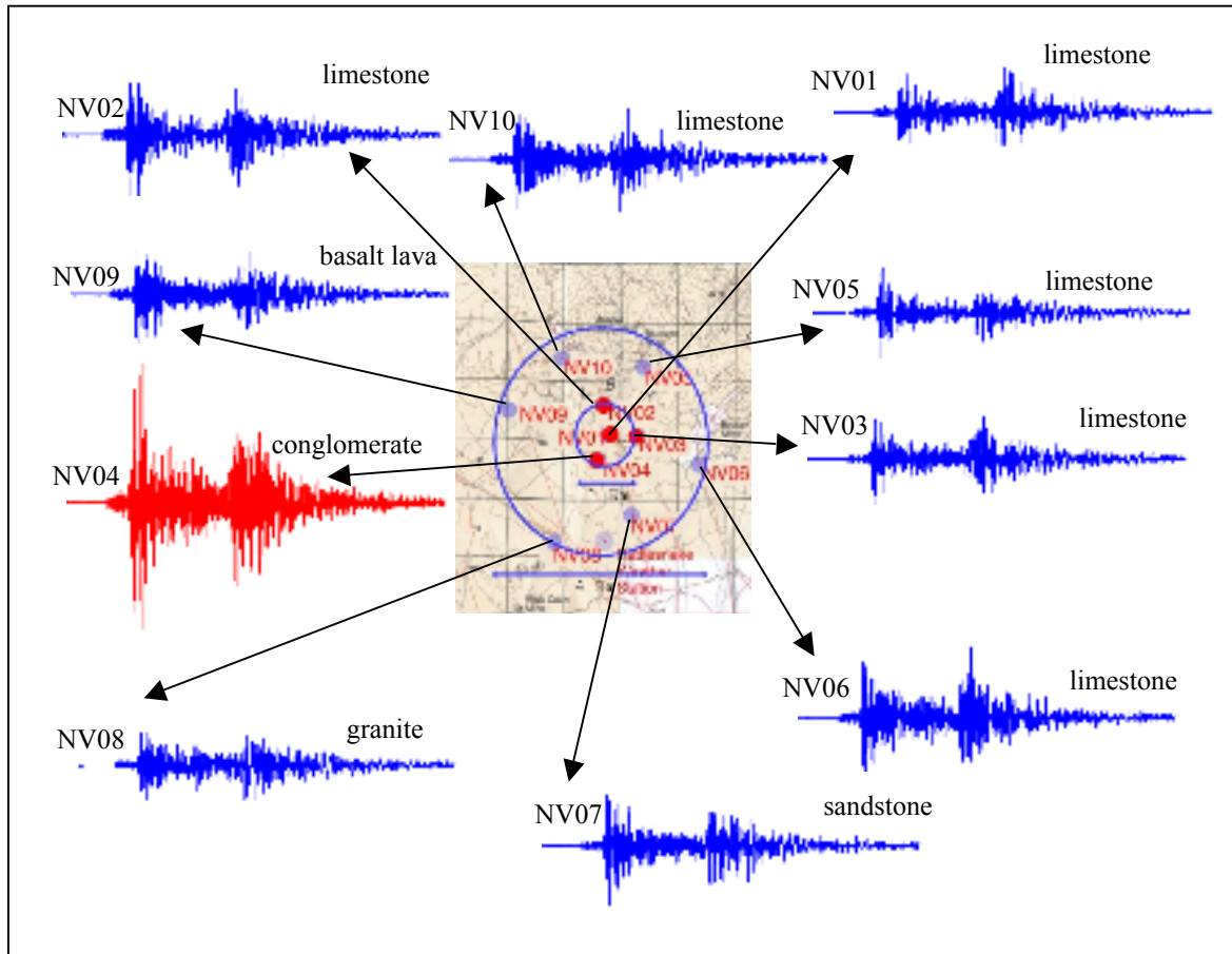
Figure 2. Detailed map of the NVAR array. The waveforms represent raw data recorded at NVAR at each of the short-period stations. The magnitude 5.7 earthquake occurred in California at a distance of 478 km. All the traces shown here are at the same scale. The red trace is channel NV04, located in Tertiary conglomerate, which exhibits the largest amplitude by a factor of three in this particular case.
