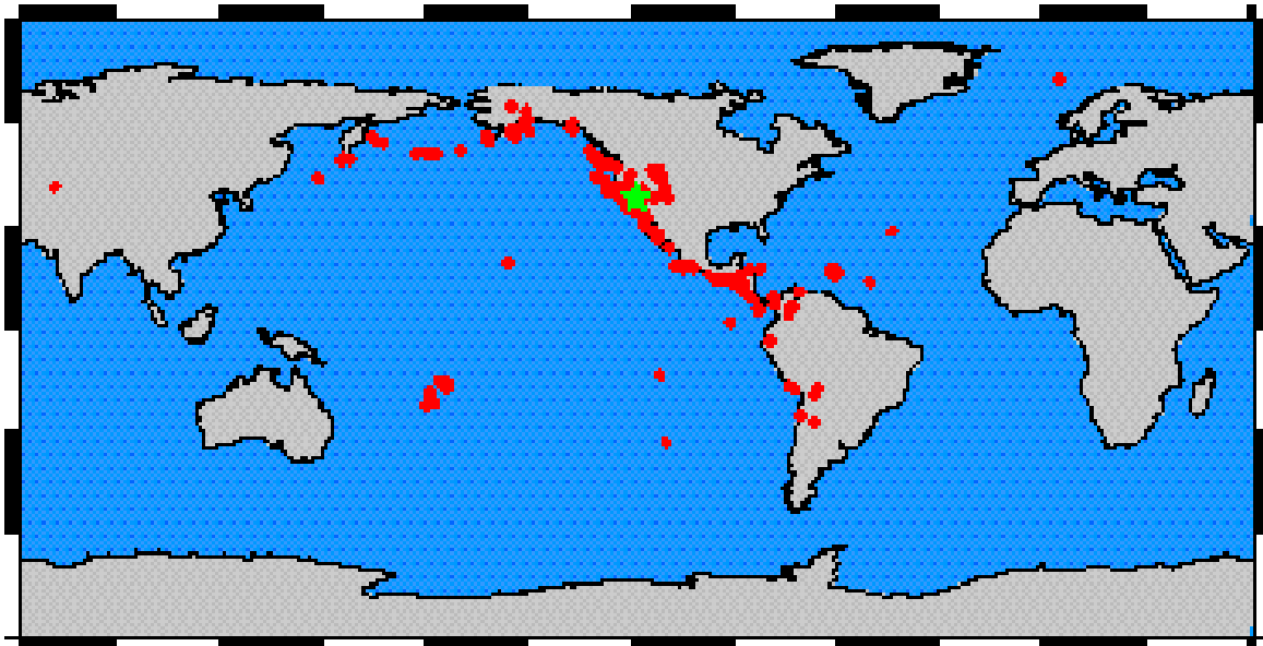
Figure 1. Position of earthquakes used in this study. The green star represents the location of the Nevada Seismic Array (NVAR)
