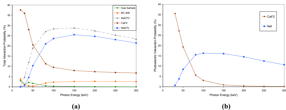
Figure 5. (a) Total interaction probability of photons with xenon gas, BC-400, \text{CaF}_2 and NaI(Tl) in the triple-layer phoswich detector (NaI(Tl)* is from the 2-layer version and is given for reference, see the text) and (b) photoelectric interaction probability of photons with \text{CaF}_2 and NaI(Tl). The figure shows the simulations for one side of the detection system.
