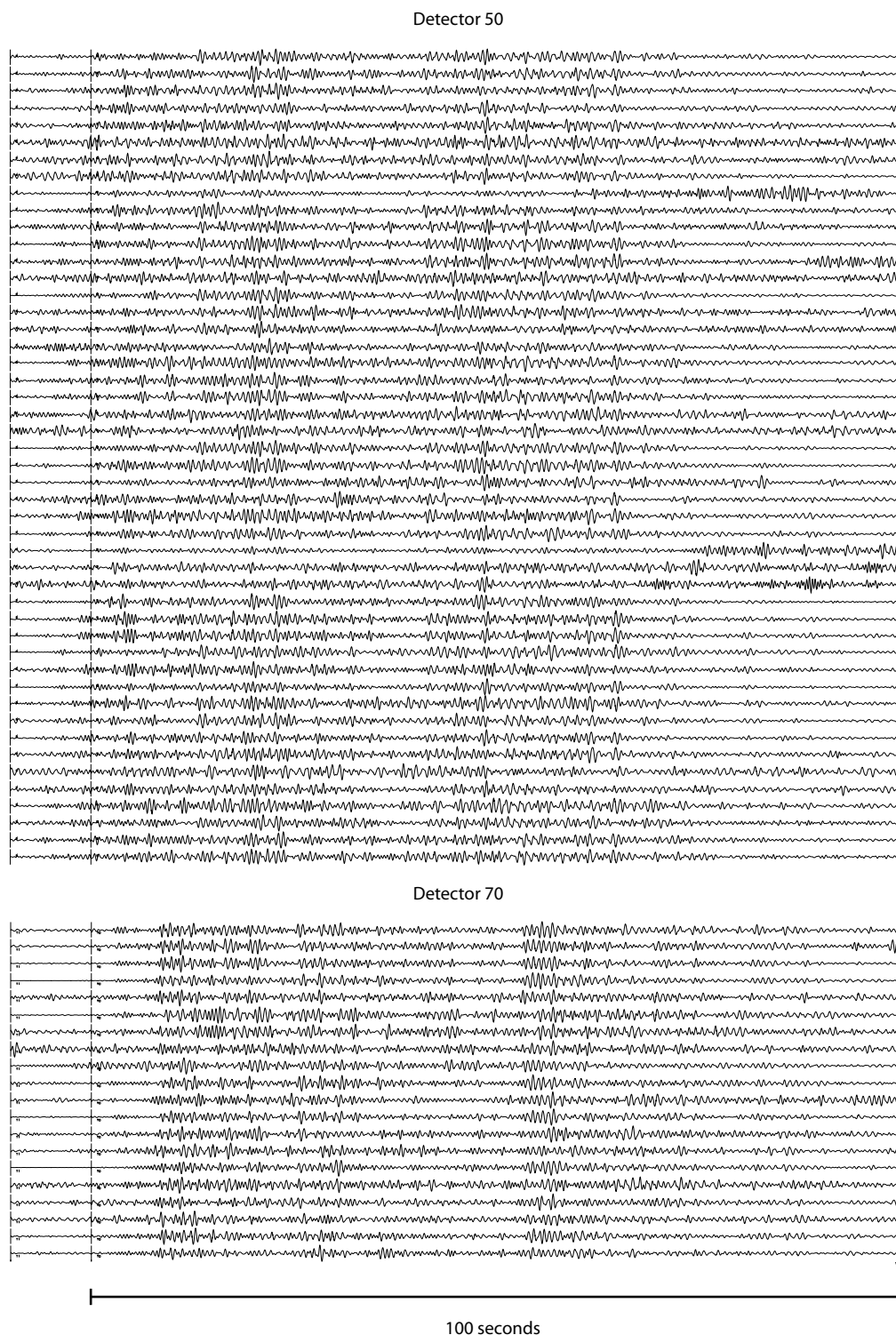
Figure 6. Two of the largest clusters of San Simeon aftershocks, automatically assembled and aligned, support our contention that efficient review by analysts would be enabled by future implementations of systems like this one.
