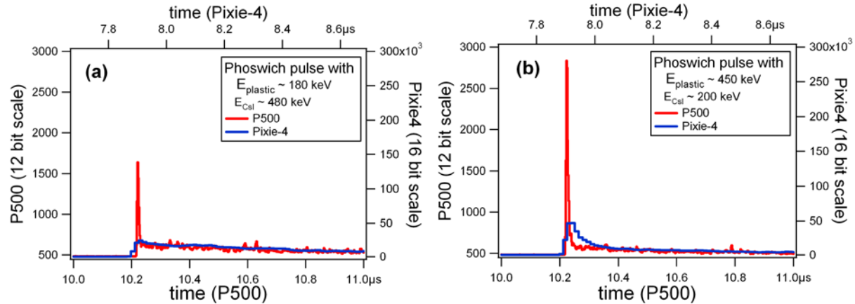
Figure 12. Phoswich waveforms captured by Pixie-4 and P500. The waveforms (a) and (b) are examples of events with energies falling into the Compton scatter line of constant energy at positions marked in Figure 11.
