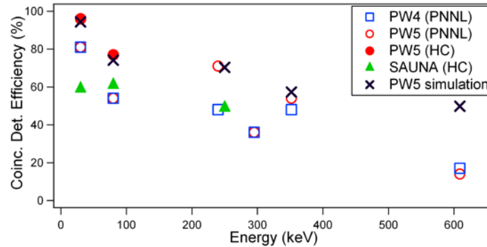
Figure 5. Coincidence detection efficiency of PW4, PW5 and a SAUNA detector installed at Health Canada. Values at 30 and 80 keV are from ^{133}Xe , not ^{131m}Xe or ^{222}Rn .
