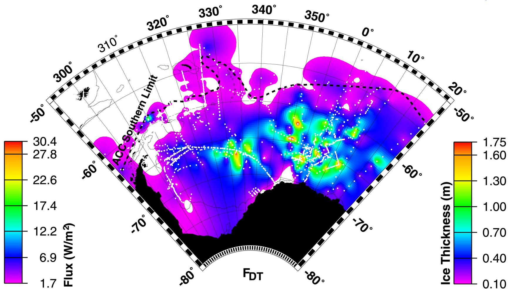
Plate 9: Average winter diffusive heat flux in units of W/m^2 and in units of ice melt over the course of a 5 month winter. This value is proportional to the thermal gradient through the pycnocline, so the spatial pattern is more robust than the absolute numbers. Contours and white areas as in Plate 8.
