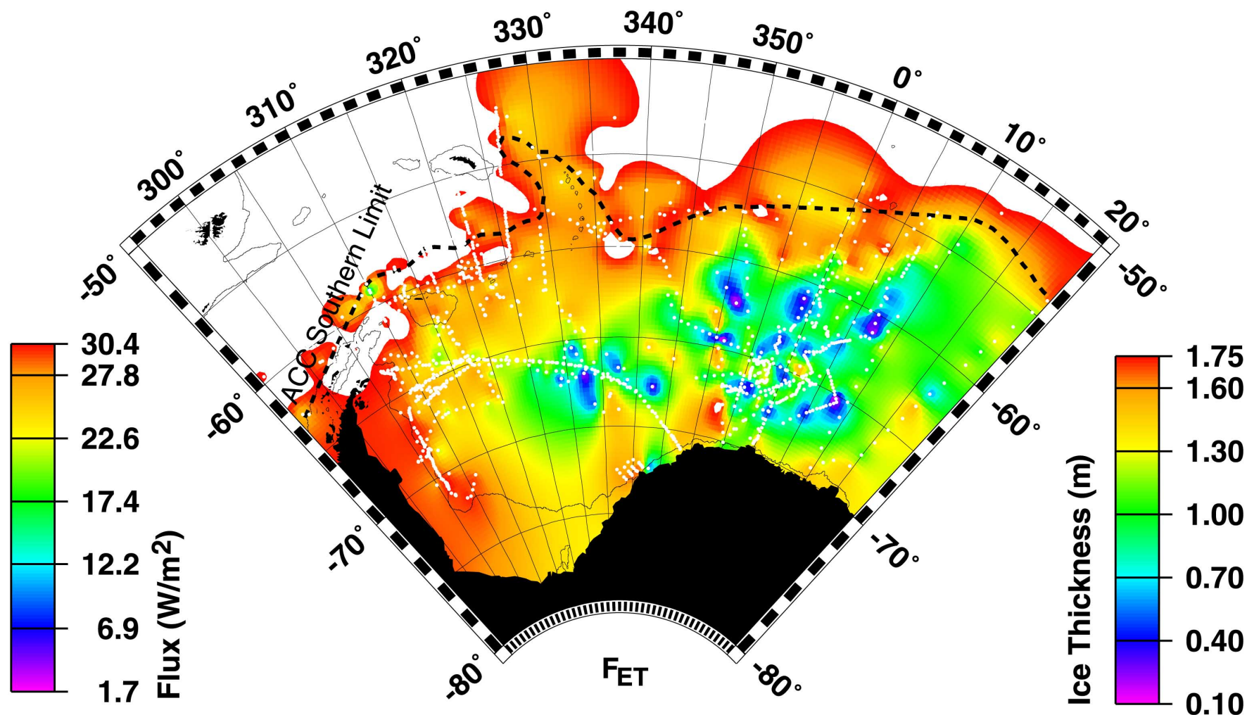
Plate 10: Average winter entrainment heat flux (units as for Plate 9). Estimate of ocean heat flux driven by entrainment in response to salinization during ice growth assuming a 35 W/m^2 air-sea heat flux. As with diffusive heat flux, spatial patterns are likely to be more robust than absolute values. Contours and white areas as in Plate 1.
