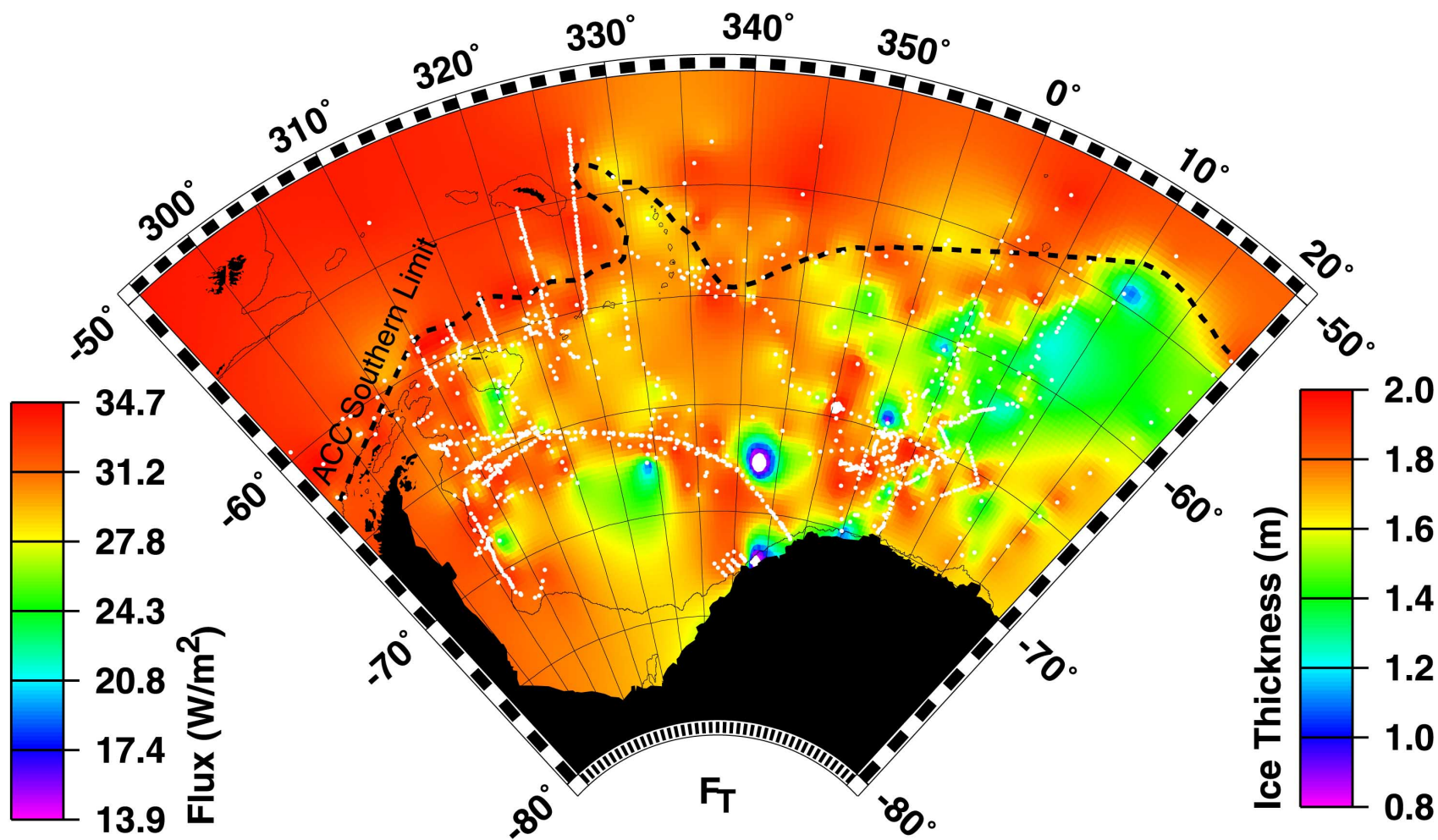
Plate 11: Total average winter ocean heat flux (units as for Plate 9). Sum of diffusive and entrainment heat fluxes. Note significant reduction in spatial variability relative to that of the two component fluxes (Plates 10 and 11). Contours and white areas as in Plate 8.
