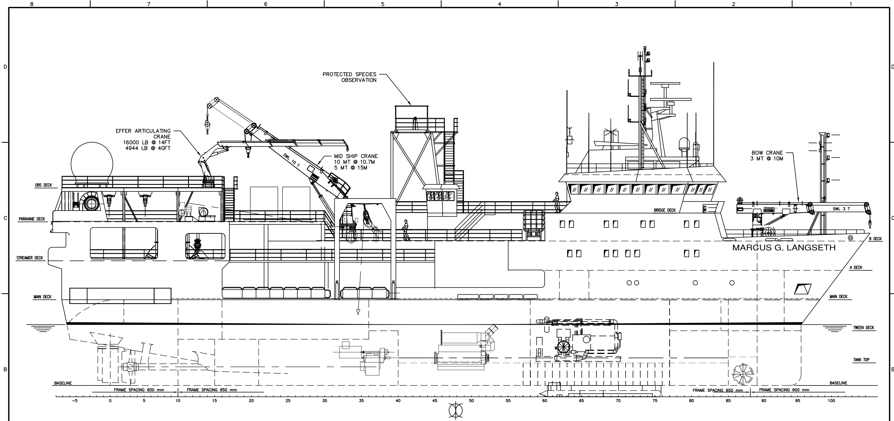
ELEVATION 1-4A OUTBOARD PROFILE 1/16"=1'-0"
