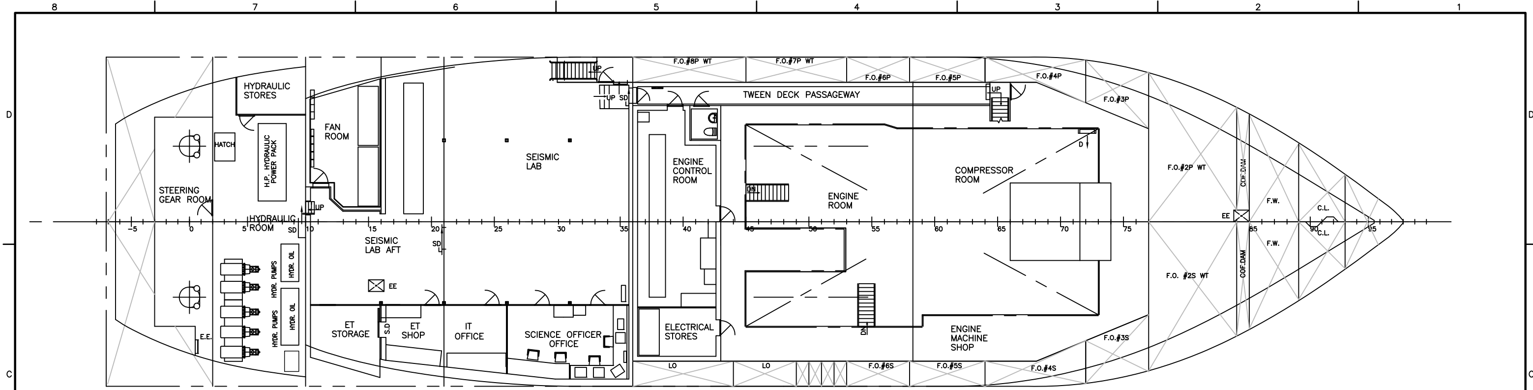
PLAN 3-4C PLATFORM DECK 1/16"=1'-0"
