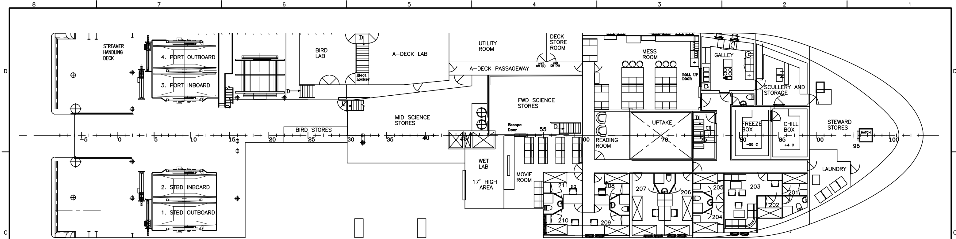
PLAN 3-4C STREAMER DECK & A DECK 1/16"=1'-0"
