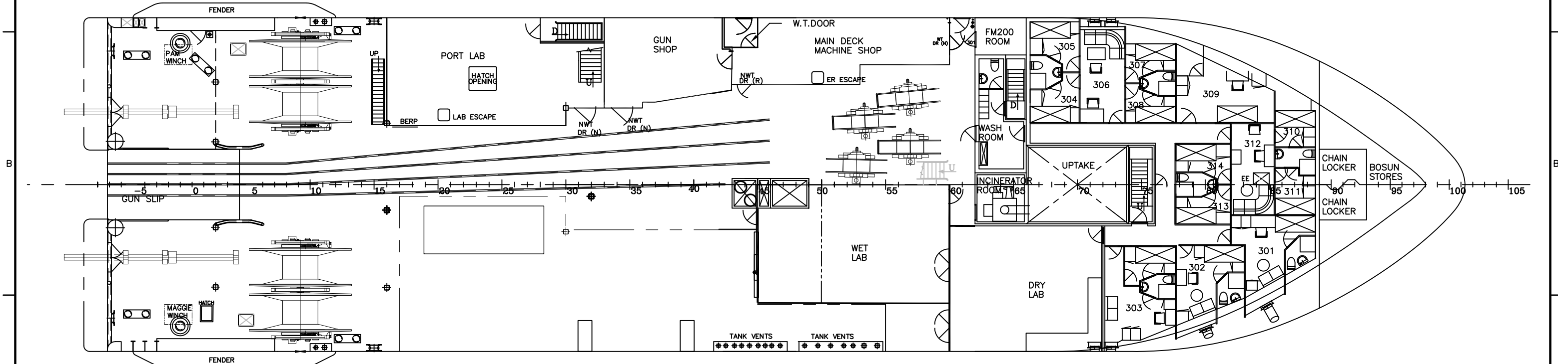
PLAN 3-4A MAIN DECK 1/16"=1'-0"
