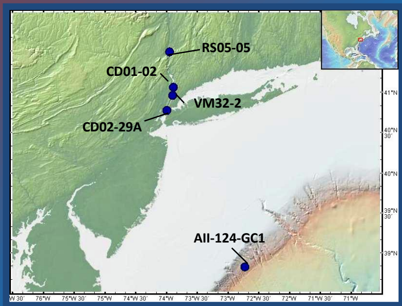
Fig. 1: GeoMapApp image detailing the locations of the Hudson River cores (CD01-02, VM32-2, CD02-29A, RS05-05) and marine core (AII-124-GC1)
