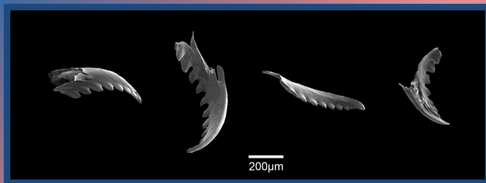
Fig. 2: Scanning Electron Microscope image of scolecodonts (polychaete annelid jaws) from Hudson River cores
