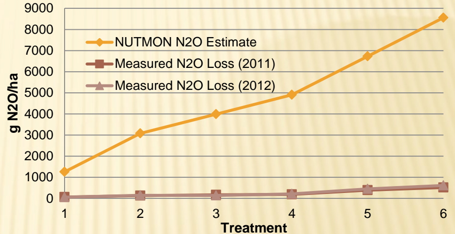
NUTMON Estimate vs. Measured Gaseous Losses
