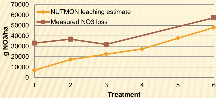
NUTMON Estimate vs. Measured Leaching Losses
