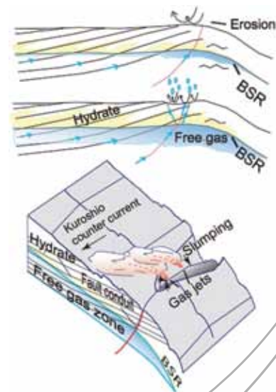
Bangs et al., 2010, Geology
