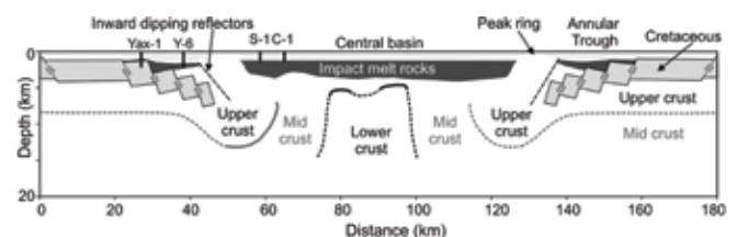
Vermeesch and Morgan, 2008, JGR
