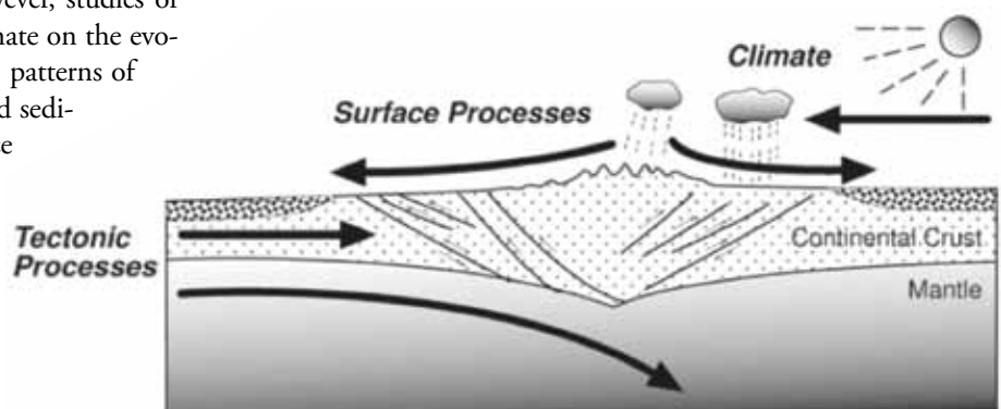
Modified from S. Willett, 1999, JGR
