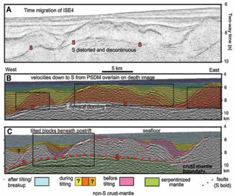
Reston et al., 2007, G-Cubed
