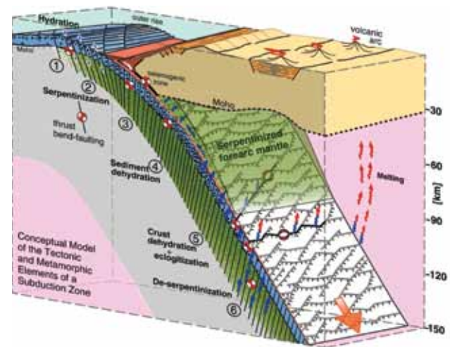
Ranero et al., 2005, G-Cubed
