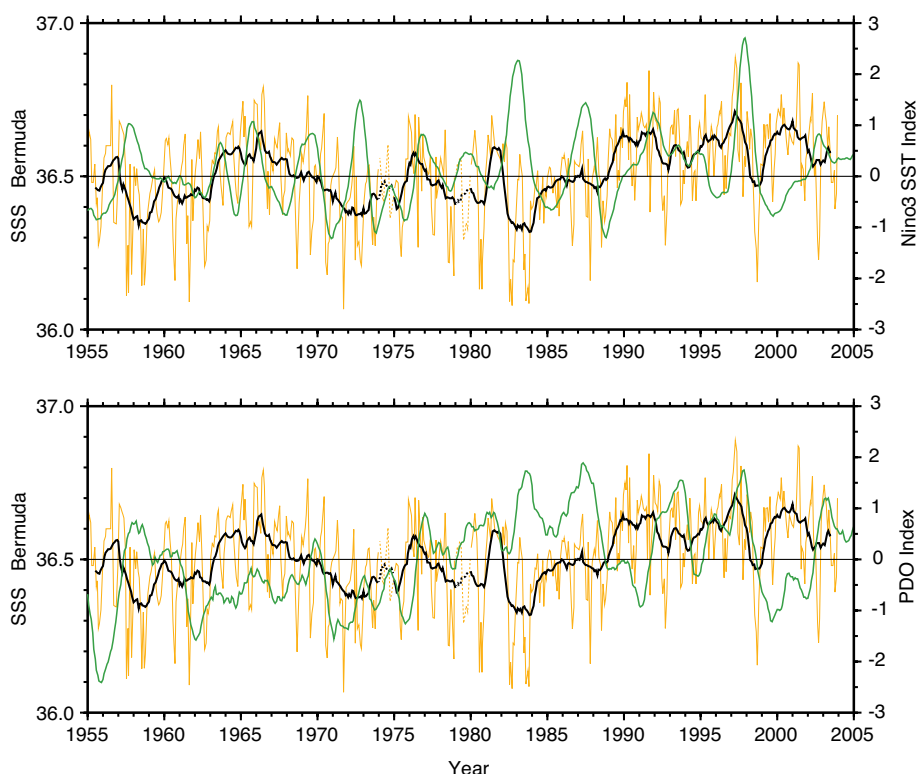
Figure 4. Monthly time series of SSS (orange line) from the combined Hydrostation S and BATS data for the period 1955–2003 (there are no data for 1979). The 12-month running mean of the combined SSS series is shown as a solid black line and a 12-month running mean of climate indices as a green line for Niño3 (upper panel) and Pacific Decadal Oscillation (PDO; lower panel).
