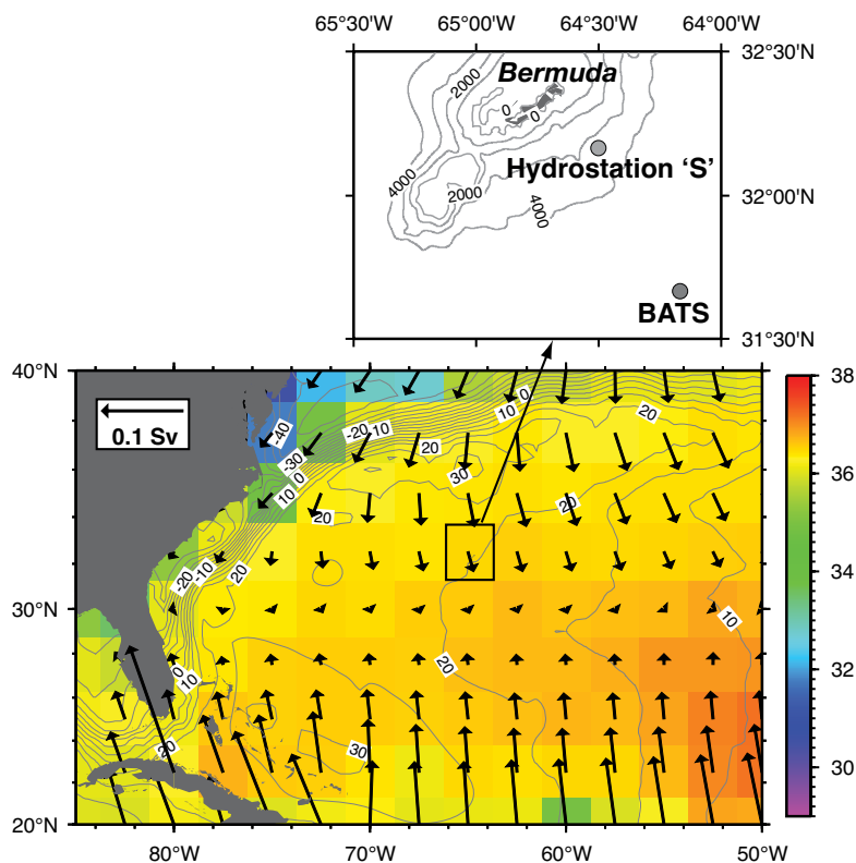
Figure 3. Ekman transport vectors in Sverdrups ( 1 \text{ Sv} = 10^6 \text{ m}^3 \text{ s}^{-1} ) and contours (every 5 cm) of mean dynamic ocean topography (MDOT) of the sea surface derived from jointly analyzed data from drifters, satellite altimetry, wind, and the GRACE (Gravity Recovery and Climate Experiment Mission) geoid model for the decade 1992–2002. The long-term mean SSS is in color. In the construction of the lower panel, Ekman transports were computed across 2.5^\circ \times 2.5^\circ latitude-longitude cells using long-term mean wind stresses based on ECMWF ERA-40 monthly data (Uppala et al., 2005). SSS (average salinity of the upper 20 m) was computed from the available hydrographic data from the World Ocean Database 2005 (WOD05; Boyer et al., 2006). Nikolai Maximenko (IPRC) and Peter Niiler (SIO) provided the 1992–2002 mean ocean dynamic topography data. The upper panel shows the location of the Bermuda Atlantic Time-series Study (BATS) and Hydrostation “S” sites in the Sargasso Sea (solid circles).
