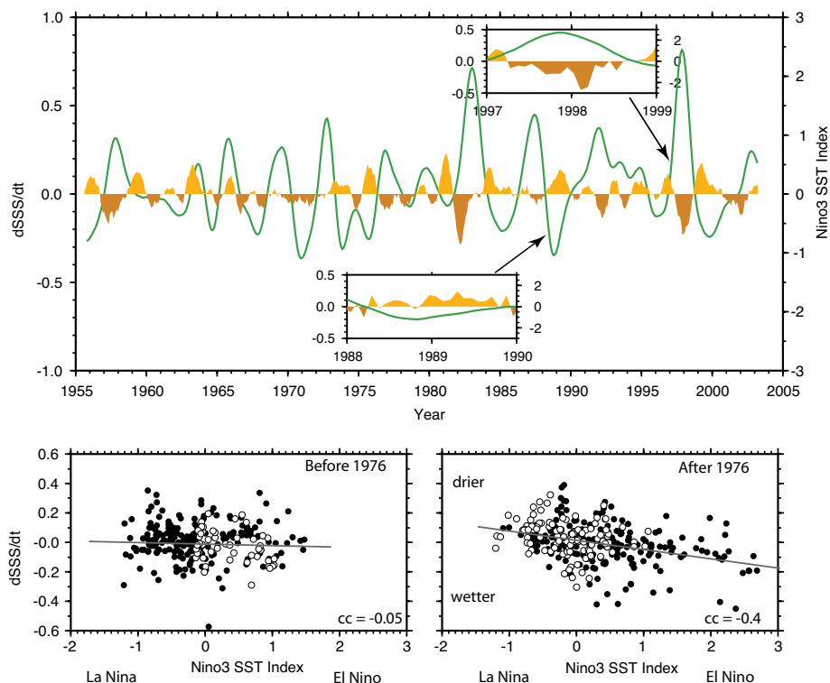
Figure 5. Upper panel: Monthly rate of change of SSS with the high-frequency fluctuations smoothed by the application of two running means, first an eight-month running mean and then a twelve-month running mean. The same procedure was done on Niño3, green line. The lighter-orange color denotes a positive rate of change of SSS values (increasing SSS with time), while brown denotes a negative rate of change (decreasing SSS with time). The two boxes in the upper panel display a more detailed view of a period of decreasing SSS, which corresponds to the strong El Niño event of 1997/1998, and increasing SSS corresponding to the strong La Niña event of 1989. For these data, a single 12-month running mean filter was applied. Lower panels: Monthly SSS change vs. Niño3 for the period 1955–1976 (left) and 1977–2003 (right). These data points are from a single 12-month running mean filter output. Open circles show positive (negative) PDO values during a negative (positive) PDO phase before (after) 1976. Correlation coefficients are indicated in the panels.
