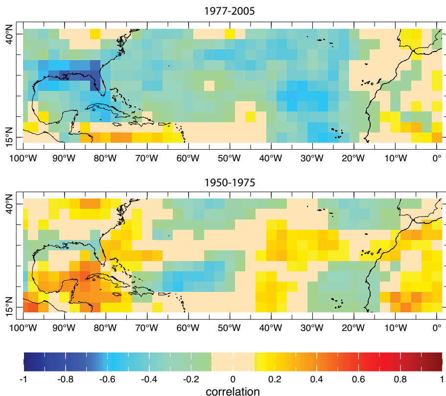
Figure 6. Winter (December-January-February) correlation maps between subtropical North Atlantic evaporation minus precipitation (E-P) and Niño3 Index for the period 1977–2005 (upper panel) and 1950–1975 (lower panel). This winter period is shown because in that season, the rainfall over the US Gulf Coast reveals the strongest correlation to ENSO. Atmospheric data are from the National Centers for Environmental Prediction.
