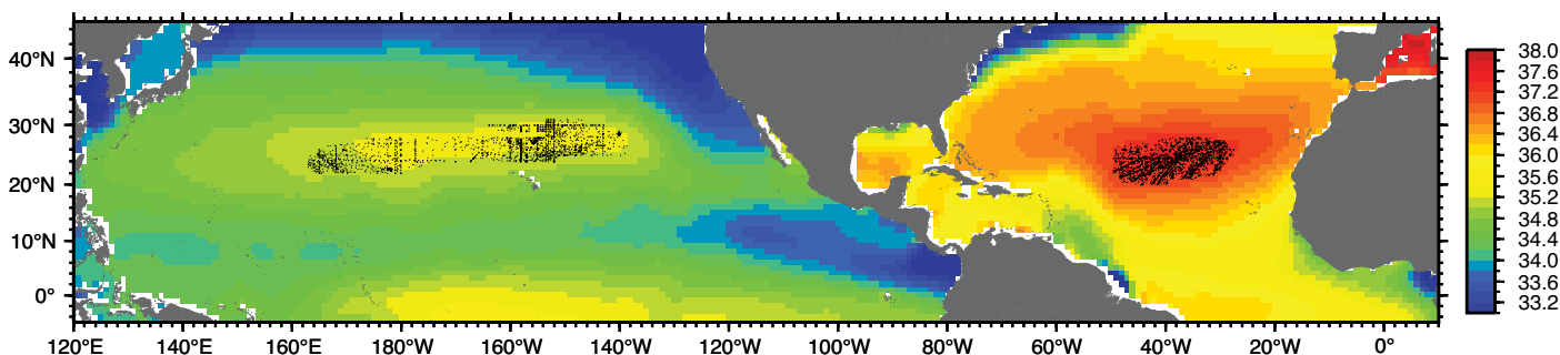
Figure 1. Annual mean sea surface salinity (SSS, defined as average salinity of the upper 20 m) from the 1° x 1° World Ocean Atlas 2005 (Boyer et al., 2006). Solid circles indicate the location of archived hydrographic stations within the North Atlantic and North Pacific subtropical gyres used to construct the SSS time series shown in Figure 2.
