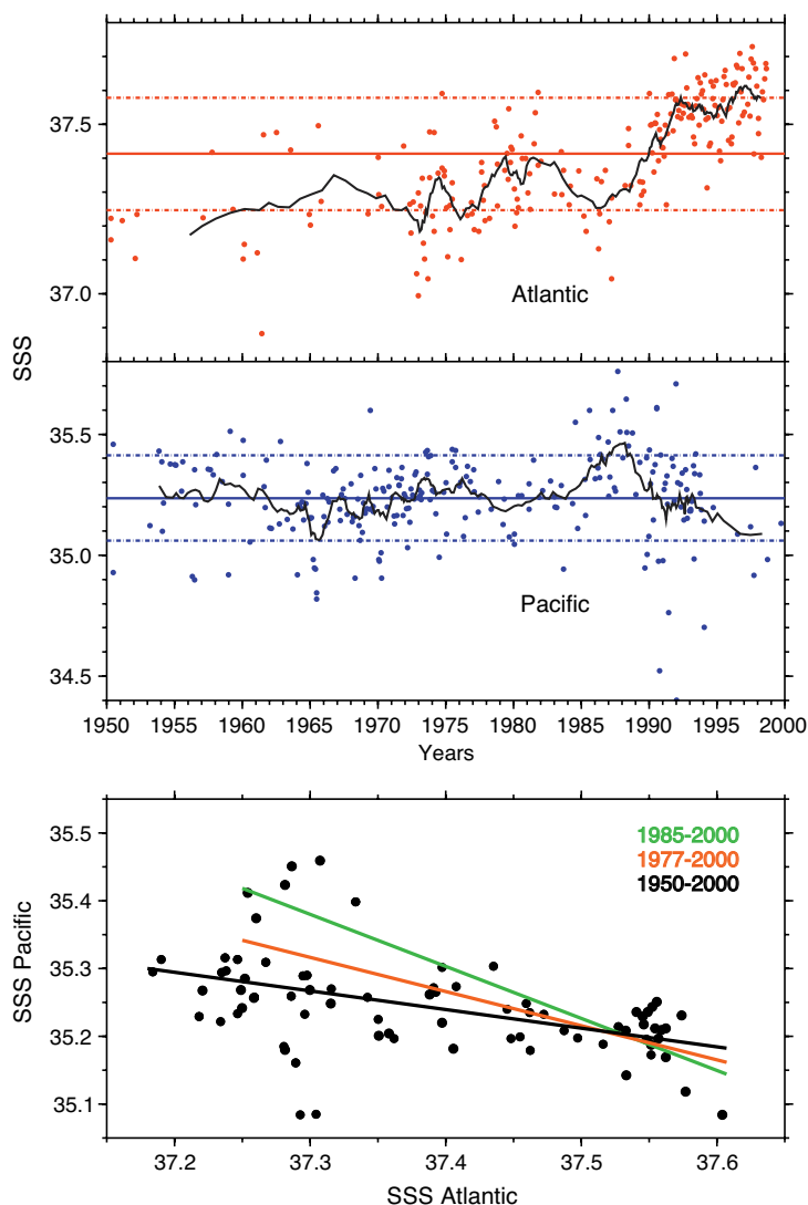
Figure 2. Upper panel: SSS time series for the central regions of the North Atlantic and North Pacific subtropical gyres shown in Figure 1. Circles represent the monthly averages of the data, and the solid black line is a 12-month running mean. Solid and dashed lines indicate the mean and 1 standard deviations of the monthly SSS data. Lower panel: North Pacific SSS versus North Atlantic SSS based on the 12-month running means. Solid lines represent the least-squares fit to the SSS averages for different periods.
