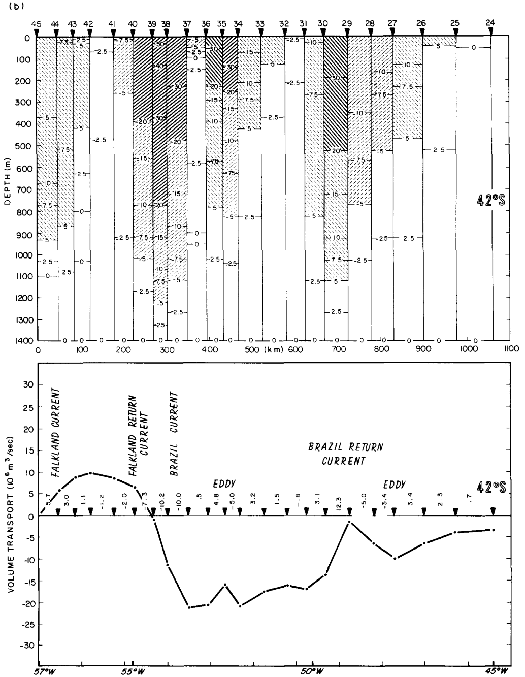
Fig. 3b. Geostrophic velocity and accumulated transport section along 42^\circ\text{S} . Same sign convention as (a).
