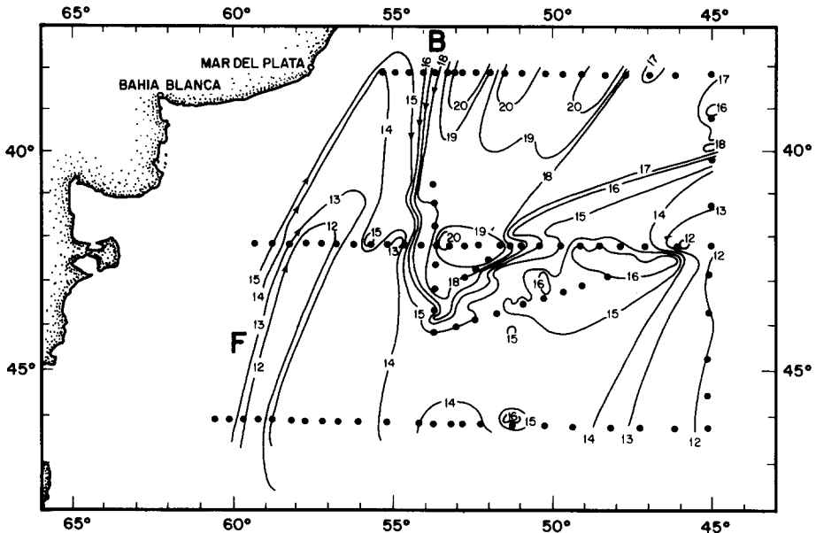
Fig. 1. Sea surface temperature from XBT and CTD stations obtained from the R.V. Atlantis II during cruise 107-3, 10 December 1979; 10 January 1980 (GUERRERO et al. , 1982). The dots represent the CTD station positions (see Fig. 2b for station numbers). A schematic representation of the Brazil (B) and Falkland (F) currents' location and direction is given by arrows superimposed on isotherms.
