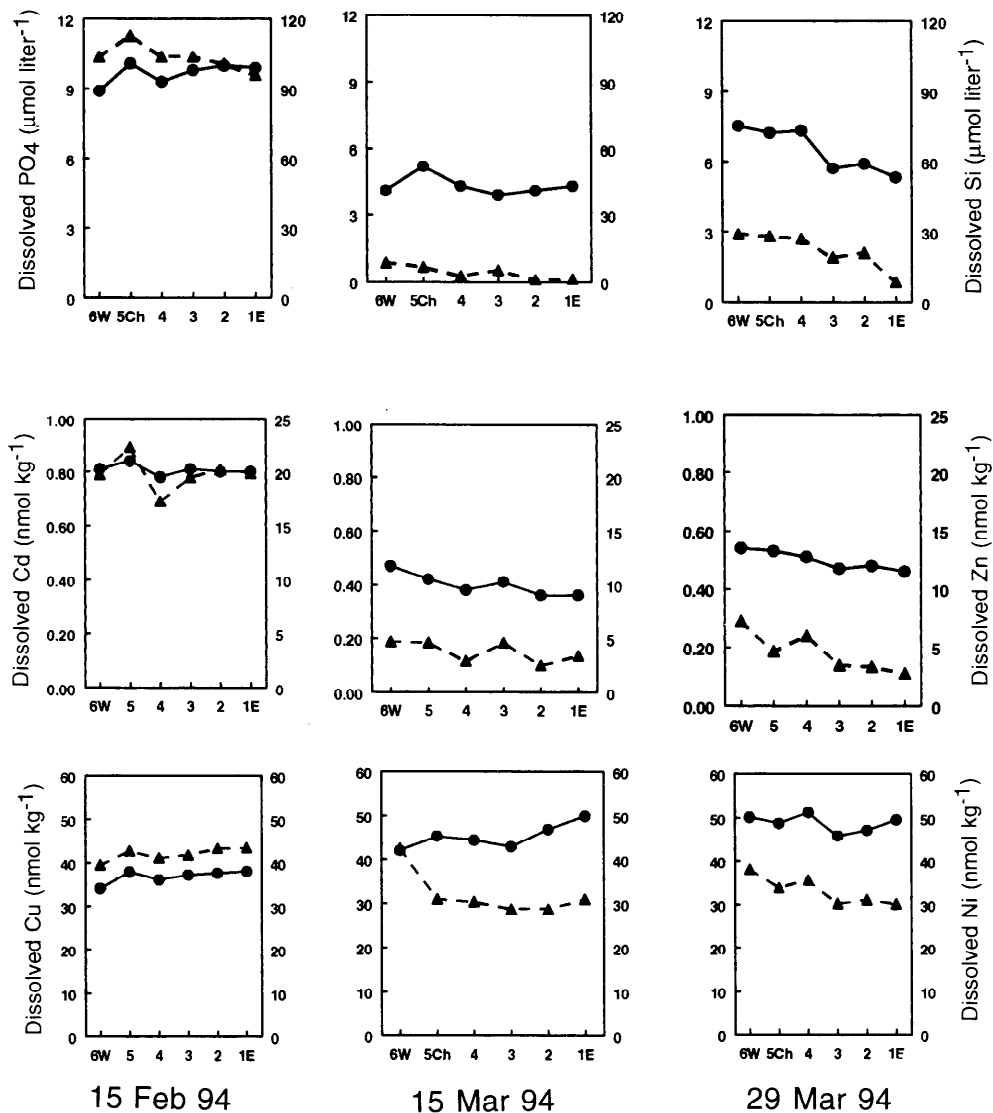
Fig. 3. Dissolved concentrations of phosphate (●) and silicate (▲), cadmium (●), zinc (▲), copper (●), and nickel (▲) observed in samples collected in a transect east (E)–west (W) in South San Francisco Bay on 15 February (before phytoplankton bloom), 15 March (midbloom), and 29 March (as the bloom receded). 5Ch is the station in the channel.
