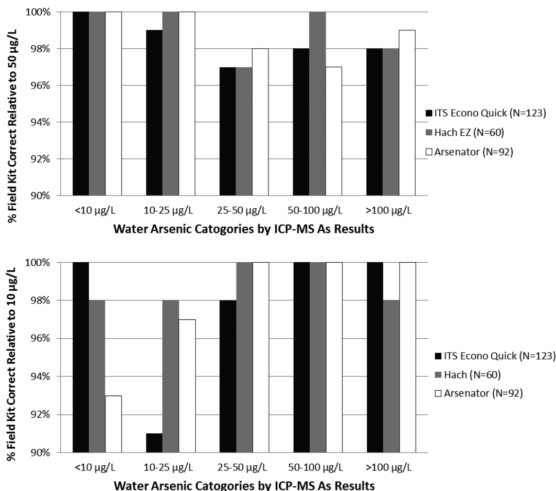
Figure 1. Comparison of ICP-MS and field kit arsenic results relative to 50 µg/L and 10 µg/L.
