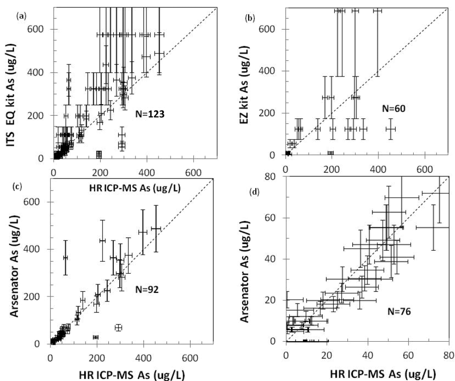
Figure 2. Comparison of As concentrations in water samples measured by inductively coupled plasma mass spectrometry (ICP-MS) compared with the outcome of field and laboratory testing with three different kits. One tubewell with an ITS EQ reading of 1000 \mu\text{g/L} and an actual concentration of 395 \mu\text{g/L} is excluded from (a) for clarity. The data in (d) are an expanded version of the same data shown in (c). Horizontal bars indicate the estimated 2-sigma errors for HR ICP-MS measurements (22). Vertical error bars in (a) and (b) indicate the full range of As concentrations ranges for the ITS EQ and the EZ kit listed in the text, respectively. Vertical errors bars in (c) and (d) correspond to an estimated error of \pm 10\% of the reported Arsenator readings. The one-to-one relationship indicating a perfect match is shown as a dotted line.
