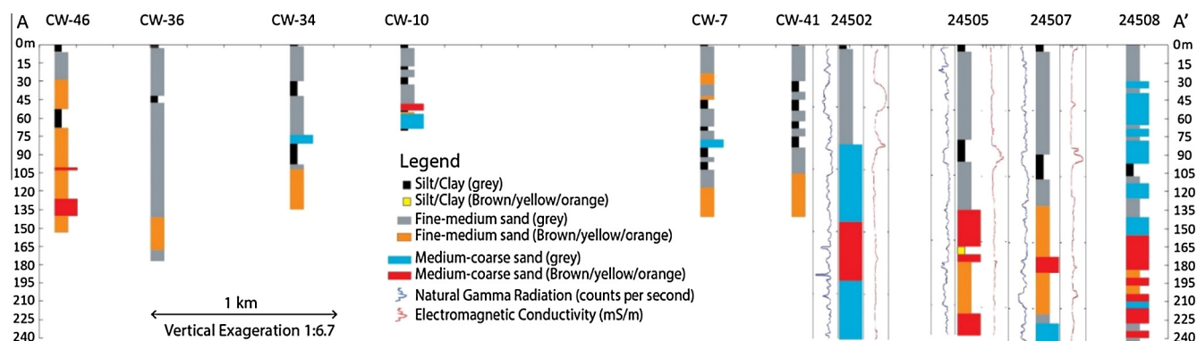
Fig. 3. Geologic cross section through Araihaaz A–A' (Fig. S1). All boreholes with ID's starting with "CW" (Community Well) were drilled using an RC method which produces excellent lithology. All other boreholes were drilled using an FC method which produces poor lithology. Electromagnetic (EM) Conductivity and Natural Gamma Radiation was recorded on some of the boreholes drilled with the FC method. Dual peaks in both the EM and Gamma logs indicate clay layers. For more information on the EM and Gamma methods see the SI.
