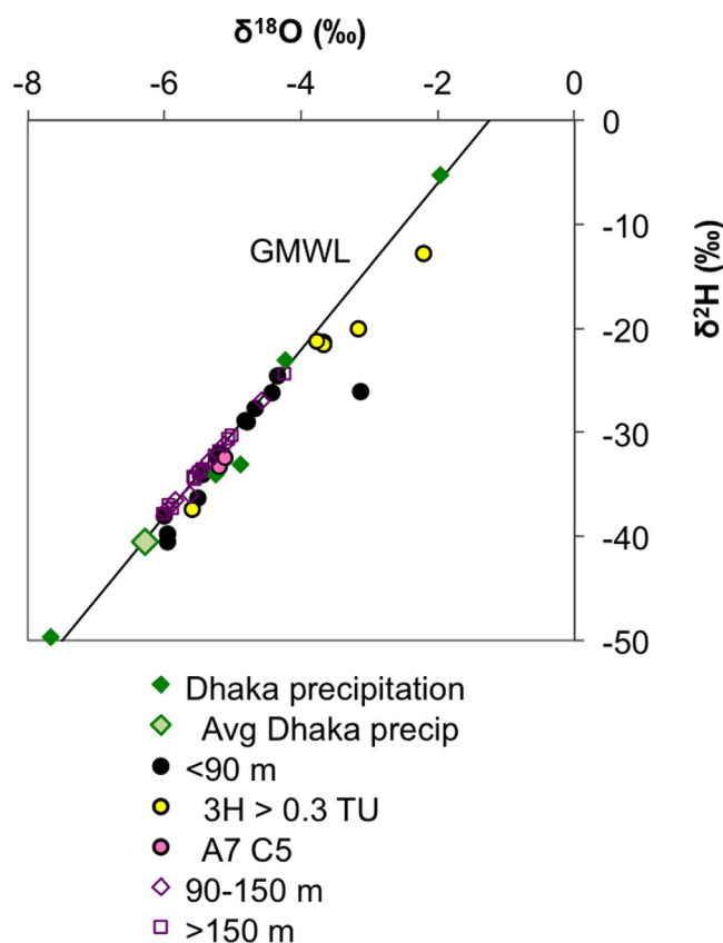
Figure 7. Water stable isotopic ( \delta^2\text{H} and \delta^{18}\text{O} ) composition of groundwater and its relationship to the global meteoric water line (GMWL) of Craig [1961]. For comparison, Dhaka precipitation and its average [Stute et al. , 2007] are also displayed. Note that the high- ^3\text{H} samples (yellow fill) plot mostly to the right of the GMWL.
