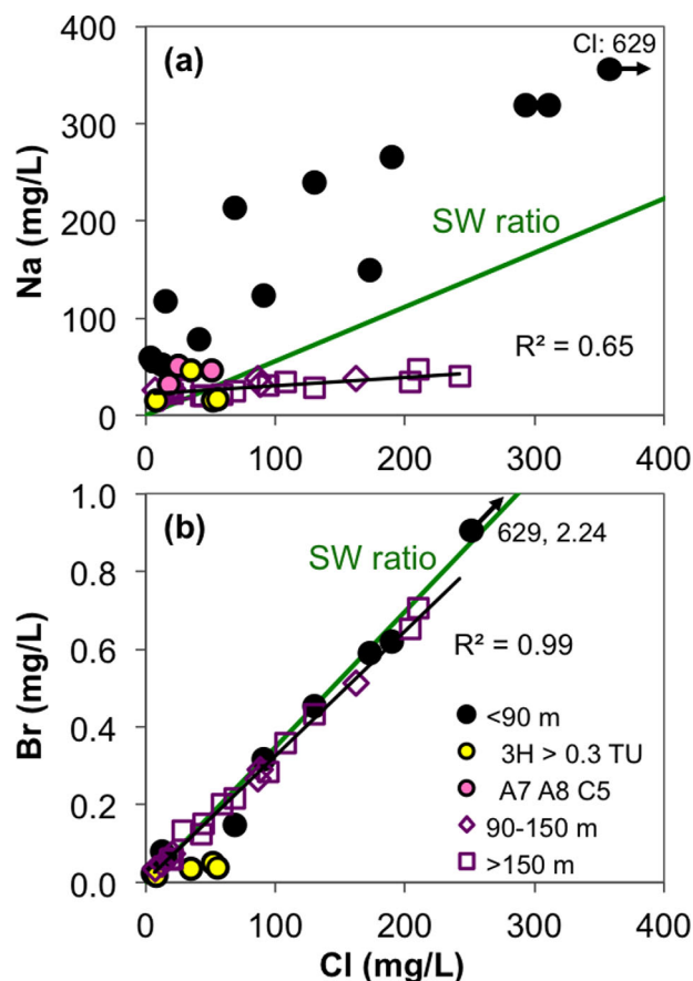
Figure 9. The correlations of (a) sodium and (b) bromide to chloride. Green lines indicate the trendlines with seawater Na/Cl and Br/Cl ratios. Black lines are the trendlines for pooled intermediate (90–150 m bgl) and deep aquifer (>150 m bgl) groundwater samples. The high Cl sample in Figure 9a actually falls on the seawater line.
