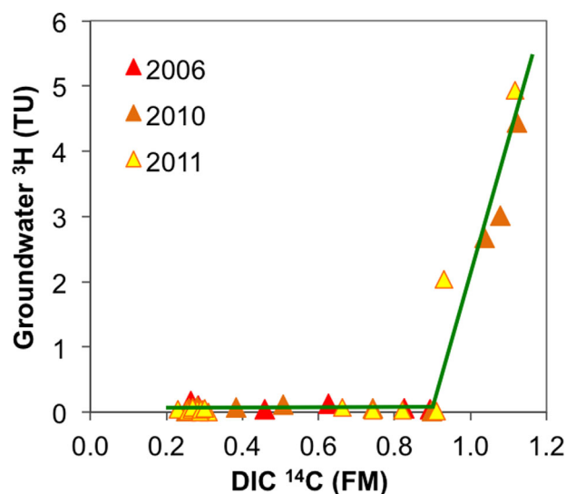
Figure 4. Empirical relationship between groundwater ^3\text{H} and ^{14}\text{C} in DIC plotted for all available samples from the shallow, low-As aquifer (<90 m bgl) with concurrently measured groundwater ^3\text{H} and ^{14}\text{C} in DIC. The initial ^{14}\text{C}_{\text{DIC}} was determined to be 0.90 FM and used to correct for the vadose zone processes before the recharge closed off from the atmosphere in \text{C}_1 and \text{C}_2 ^{14}\text{C} age calculations.
