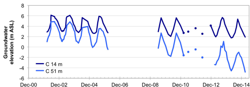
Figure 2. Hydrographs of a very shallow, high-arsenic well (14 m bgl) and a shallow-depth, low-arsenic well (C5 in this study, 51 m bgl) at the location of multilevel nest C, designated by the large blue square in Figure 1a. Hydraulic head data since 2001 indicate a steadily declining water level of the deeper, low-As well, and thus an increasing downward vertical hydraulic gradient between the shallowest and the deepest wells at this site.
