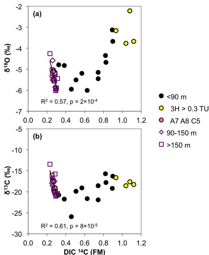
Figure 8. The relationship of (a) water \delta^{18}\text{O} and (b) DIC \delta^{13}\text{C} with ^{14}\text{C} in DIC. The trend-lines, R^2 , and p values for pooled intermediate (90–150 m bgl) and deep aquifer (>150 m bgl) samples are indicated. A similar pattern to Figure 8a is also observed for \delta^2\text{H} (not shown, R^2 = 0.60 and p = 1 \times 10^{-4} ).
