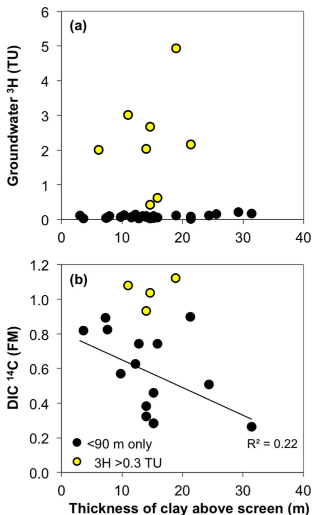
Figure 10. The relationship between groundwater (a) 3 H and (b) 14 C versus the total thickness of clay in lithologies of the shallow low-As wells. For samples where multiple measurements were made, the latest non-negative values of 3 H are shown in Figure 10a and the 14 C values from 2010 are displayed in Figure 10b. The high 3 H samples (>0.3 TU, yellow fill) were excluded from the 14 C trendline with clay thickness shown in Figure 10b.
