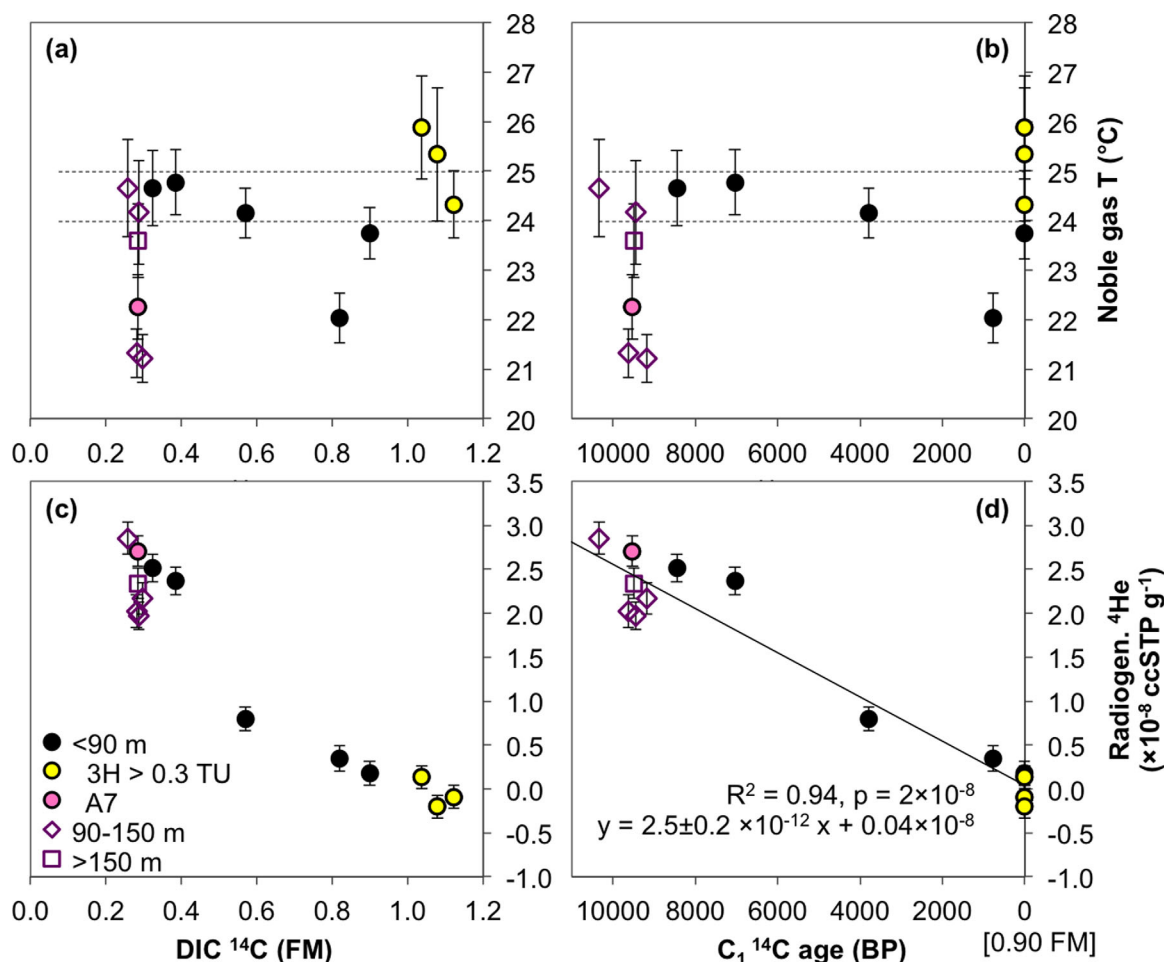
Figure 5. Noble gas temperatures and radiogenic (“excess”) He plotted against ^{14}\text{C} measured in DIC (a and c), and corrected \text{C}_1 ^{14}\text{C} ages (b and d). Noble gas temperatures, corresponding to temperatures at the time of recharge, and radiogenic He were estimated by Taf-1 model fit to the measured noble gas data. Only the samples where model converged are plotted. The errors indicated by vertical error bars combine the analytical error with model fit uncertainty. Only one sample per well is shown; where multiple noble gas measurements were made, those with the best noble gas model fit are displayed. Dashed lines in Figures 5a and 5b mark the 95% confidence interval of the average noble gas temperatures of shallow samples, excluding the two outliers at approximately 22^{\circ}\text{C} . The trend linking radiogenic He to \text{C}_1 ^{14}\text{C} ages was calculated for combined shallow, intermediate, and deep groundwater samples.
