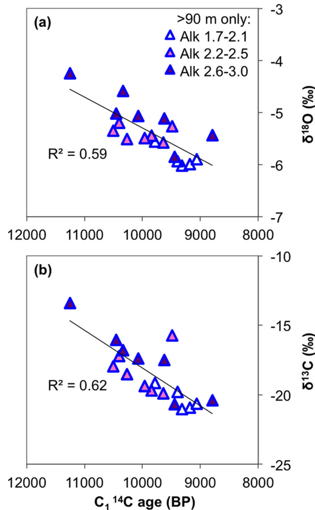
Figure 11. Plots of (a) \delta^{18}\text{O} and (b) \delta^{13}\text{C}_{\text{DIC}} against the C_1 ^{14}\text{C} age in intermediate and deep groundwater only (samples from >90 m bgl), with an added third dimension of alkalinity. The units of alkalinity concentrations shown in the legend are mEq/L, and the three concentration ranges were selected based on the spread of data values. The overall trendlines for pooled intermediate and deep samples and their R^2 values are displayed.
