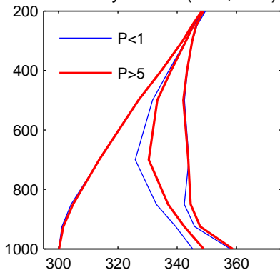
NCEP2
