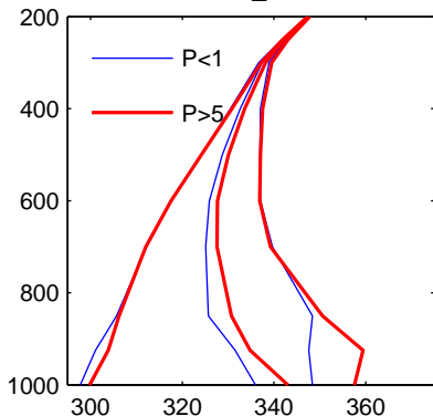
GFDL_AM2
