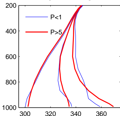
CAM2wRAS
