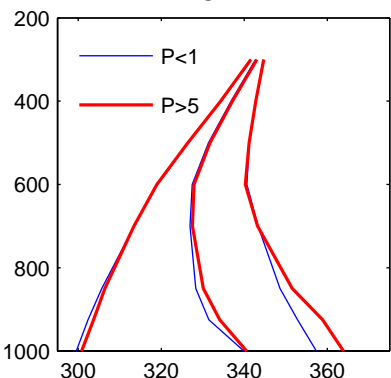
NCEP1
