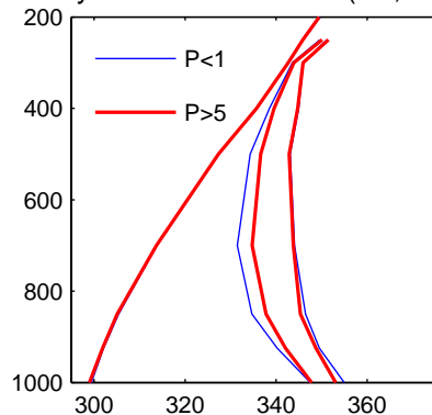
ERA40
