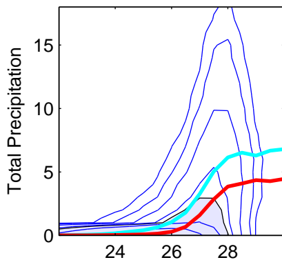
CAM
