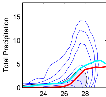
NCEP-NCAR Reanalysis
