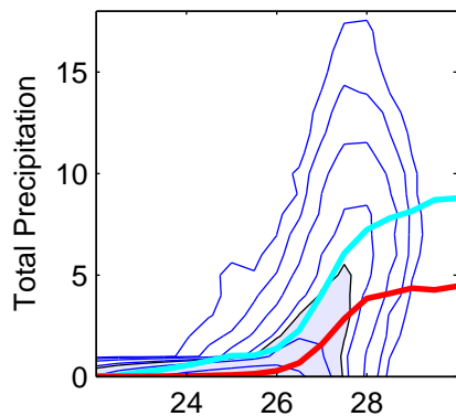
ECHAM4.5
