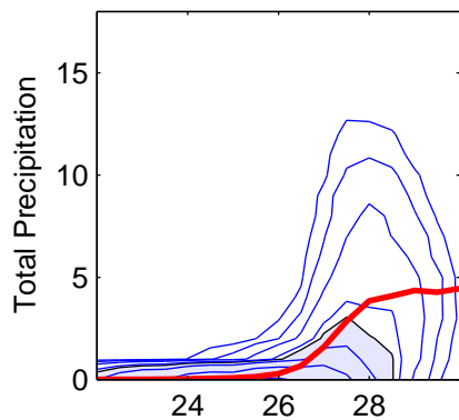
ERA40
