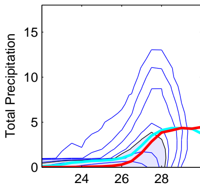
NCEP Reanalysis 2
