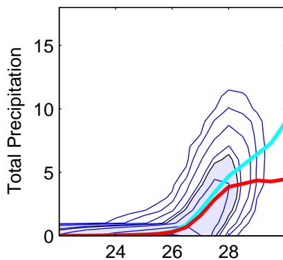
GFDL_AM2
