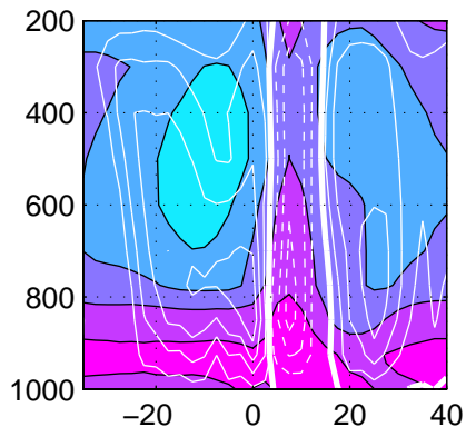
ECHAM4.5
