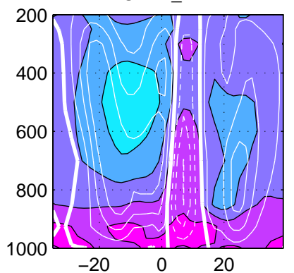
GFDL_AM2
