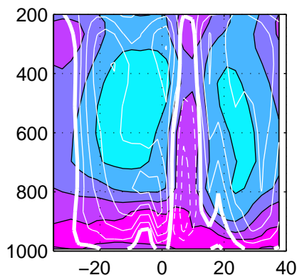
GFDL_AM2
