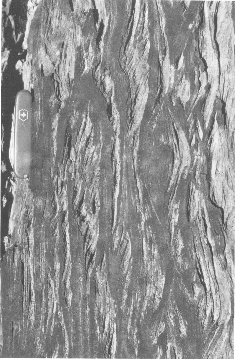
Fig. 7. Examples of hummocky cross-stratification (A) and combined-flow ripples (B) from the lower part of the Fortress Hill canyon complex.
