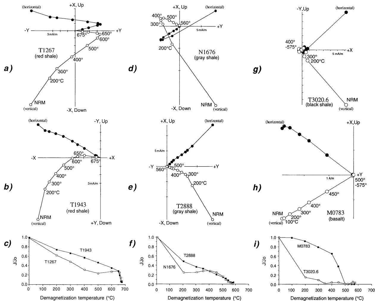
Figure 4. Vector end-point diagrams and normalized decay curves illustrating thermal demagnetization of NRM of representative samples and lithologies from NBCP drill cores. Horizontal coordinates have arbitrary azimuth; vertical coordinates correspond to drill core axis. Samples are identified with first letter of drill site and footage.
