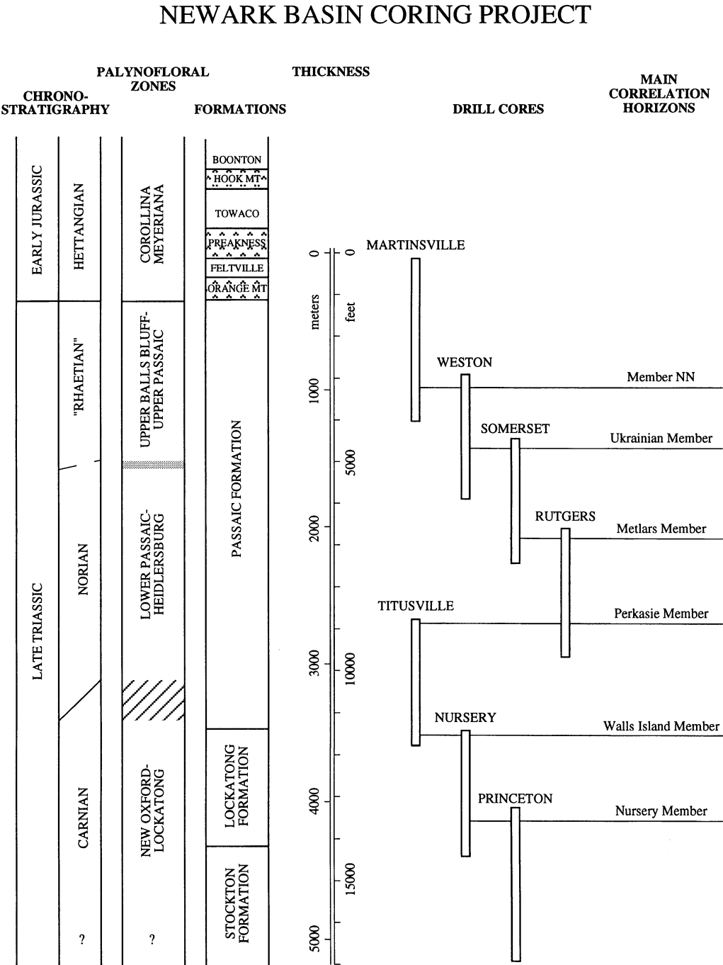
Figure 2. Stratigraphy of the Newark Basin and the section recovered by coring at the seven NBCP sites and a series of Army Corps of Engineers (ACE) cores [Fedosh and Smoot, 1988]. Thickness scale is the nominal aggregate length of stratigraphically overlapping NBCP drill cores linked by main correlation horizons. Palynofloral zonation is from Cornet [1977, 1993] and Cornet and Olsen [1985].
