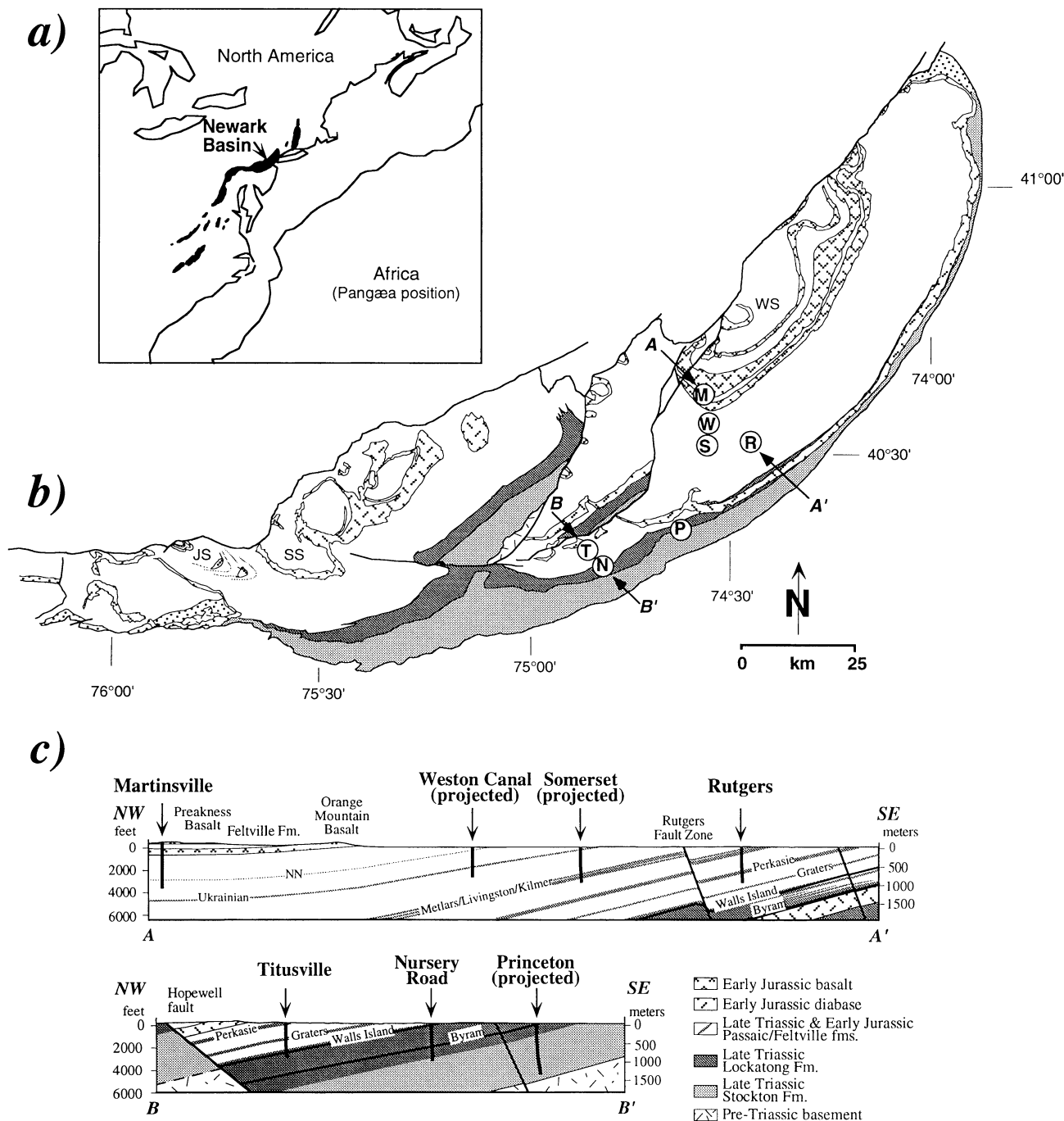
Figure 1. (a) Location of the Newark Basin among other early Mesozoic rift basins (dark shading) in eastern North America which is shown in a predrift (Pangea) continental configuration with respect to Africa. (b) Geological sketch map of the Newark Basin with the location of Newark Basin Coring Project drill sites indicated by the circled first letter of the site name. Other localities referred to in the text are WS, Watching syncline; SS, Sassamansville syncline; JS, Jacksonwald syncline. (c) Cross sections showing positions of NBCP drill sites projected onto A-A' and B-B' of Figure 1b.
