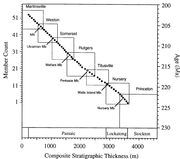
Figure 19. Lithostratigraphic members numbered sequentially from the base of the Lockatong Formation to the top of the Passaic Formation as a function of stratigraphic thickness of the composite section (normalized to the Rutgers drill core). Note that T-U is assumed to be two separate members even though not readily differentiated lithologically in the Rutgers drill core. Conversion to time is based on an age for the Triassic/Jurassic boundary (within member number 53, Exeter Member) of 202 Ma and assuming that each member represents a 413-kyr McLaughlin cycle. Boxes show the stratigraphic range encompassed within each drill core; key members in common between drill cores are labeled for reference.
