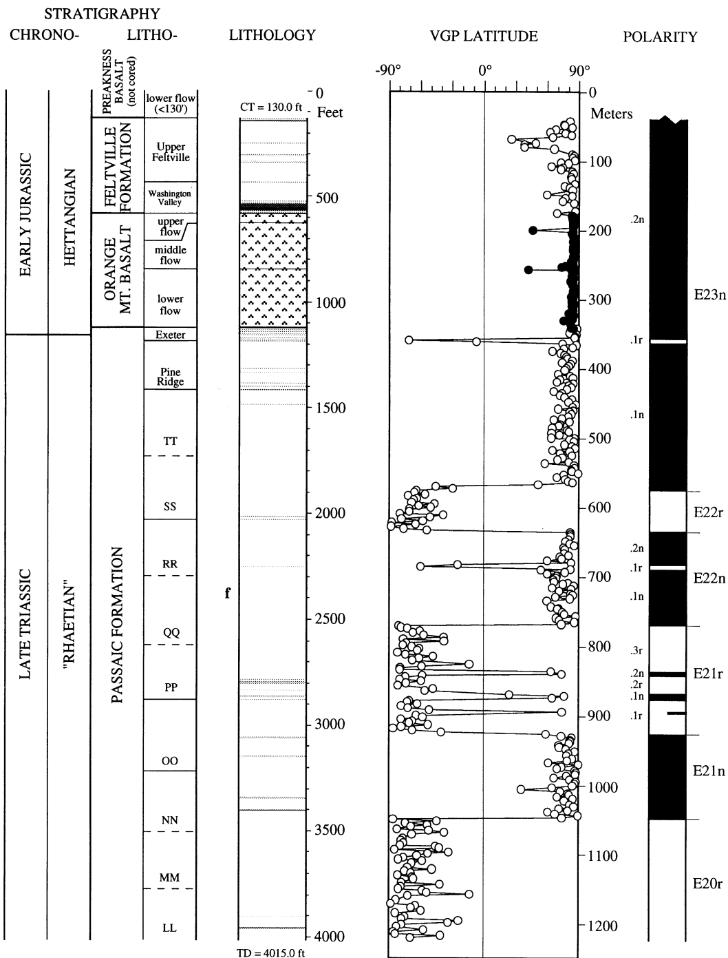
Figure 15. Physical stratigraphy, lithology, and magnetostratigraphy of the Martinsville drill core. Conventions as in Figure 9. Lithology column includes basalt.
