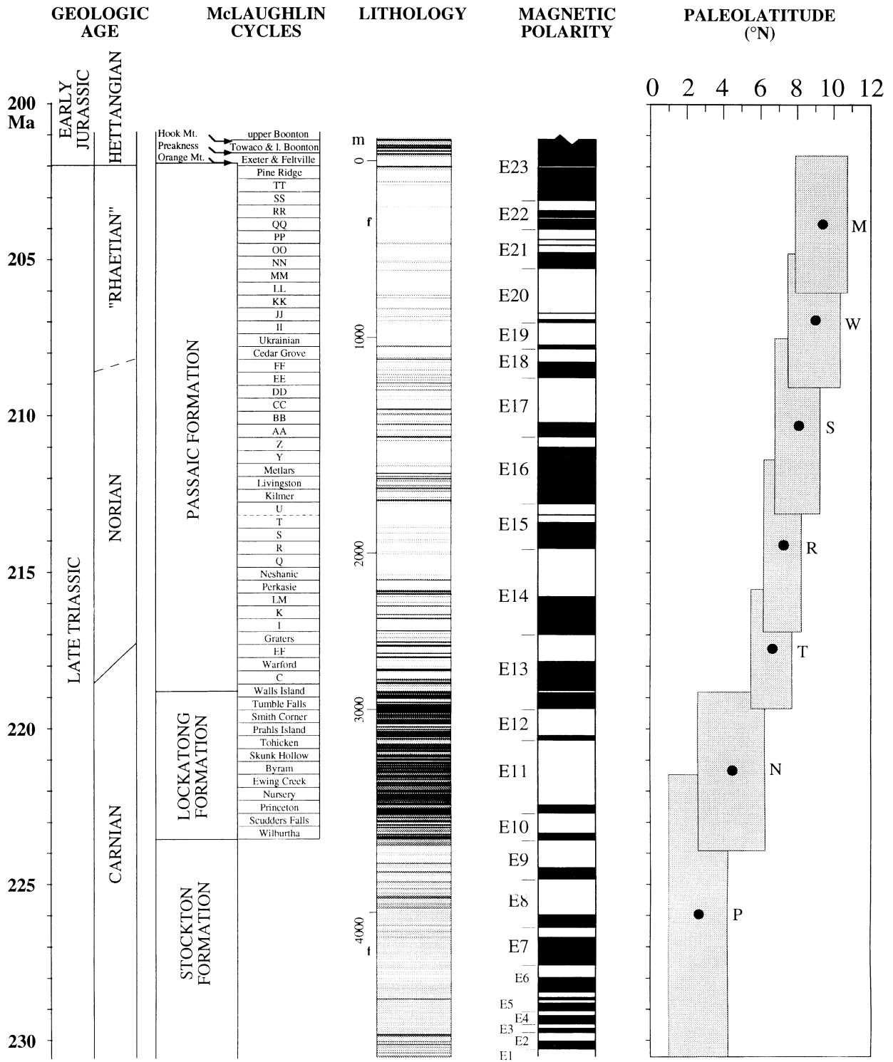
Figure 20. Newark Basin composite section transformed into a chronostratigraphy, using an age of 202 Ma for the Triassic/Jurassic boundary and assuming that the lithologic members (McLaughlin cycles) each represent 413 kyr and that the Stockton Formation has a sedimentation rate of 140 m/m.y. Conventions as described for Figure 9. Note that T-U is assumed to be two separate members even though not readily differentiated lithologically in the Rutgers drill core. Magnetic polarity column includes results for the earliest Jurassic not covered by the NBCP drill cores from McIntosh et al. [1985], Witte and Kent [1990], and Witte et al. [1991]. Mean paleolatitudes (solid circles) and associated 95% confidence intervals (width of shaded boxes) are based on the mean characteristic magnetizations for the NBCP drill cores whose stratigraphic intervals are indicated by the heights of the shaded boxes.
