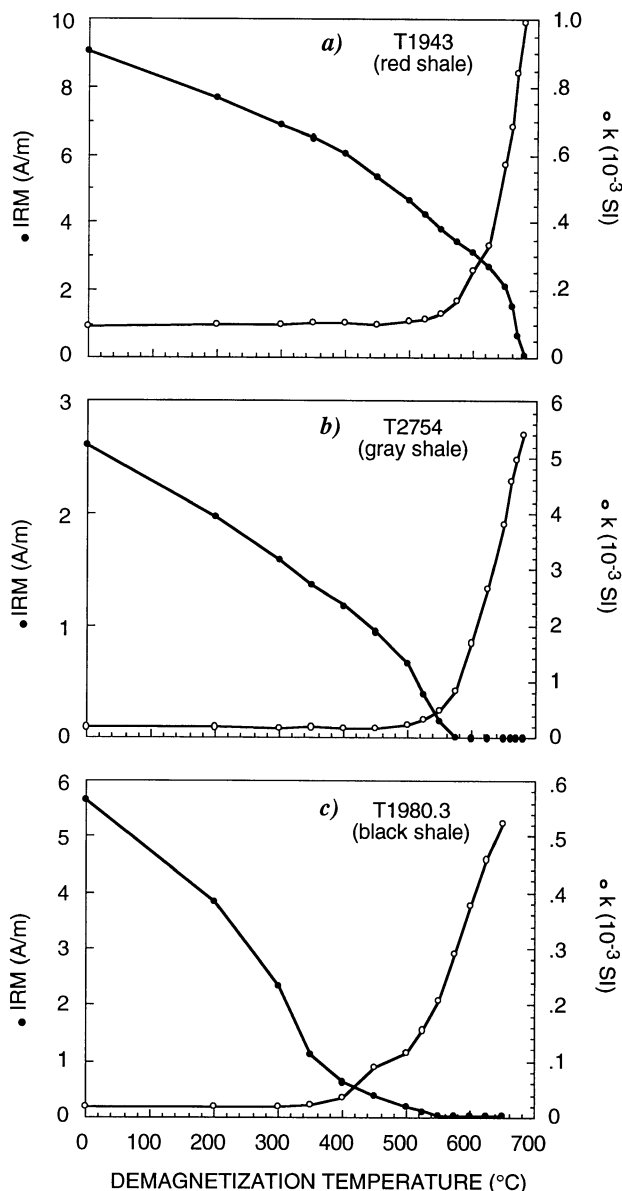
Figure 5. Thermal demagnetization of IRM (1 T) of representative sedimentary samples from NBSP drill cores. Samples are identified with first letter of drill site and footage.
