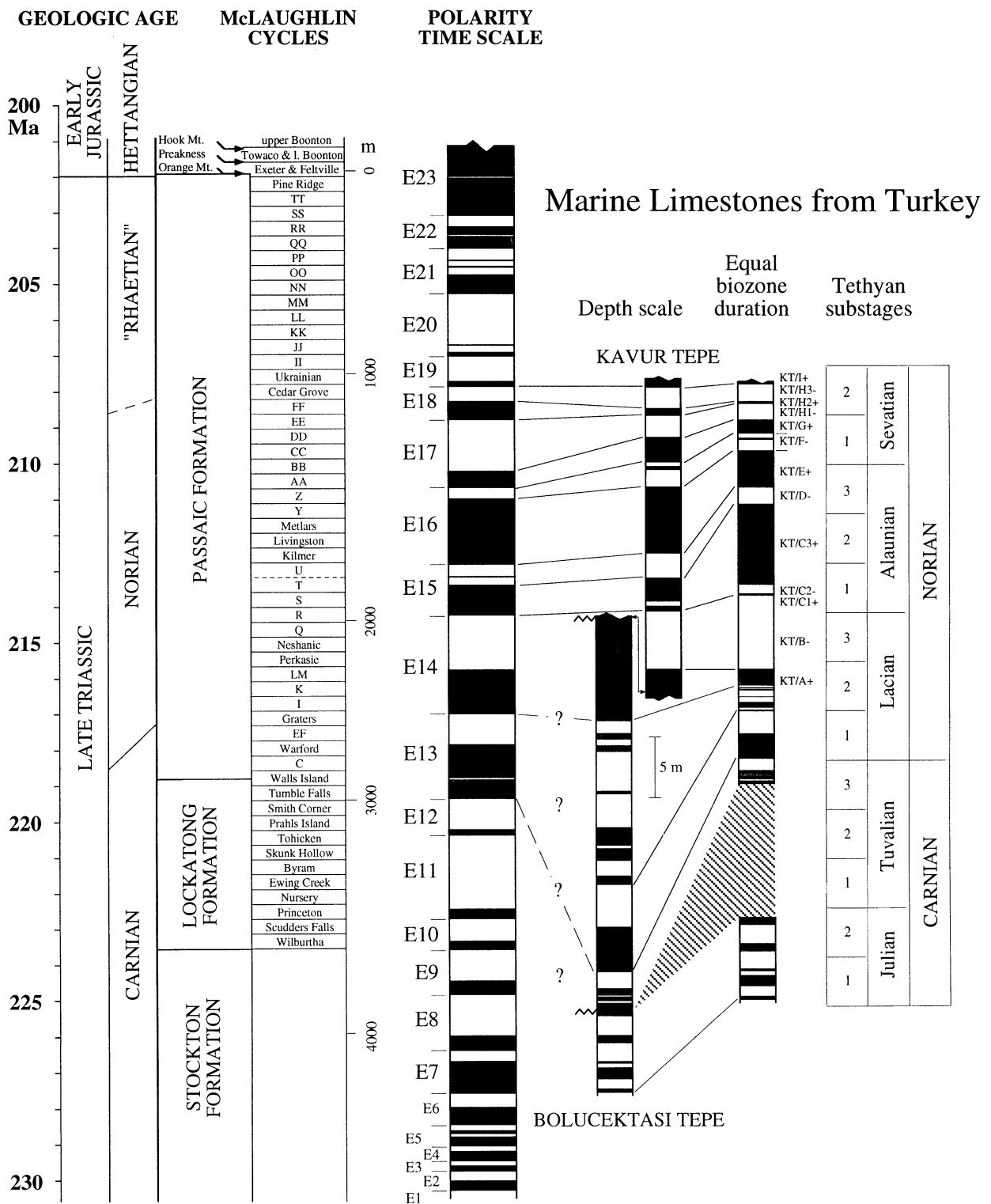
Figure 22. Magnetostratigraphies from marine limestone sections from Turkey (Bolücektasi Tepe [Gallet et al., 1992] and Kavour Tepe [Gallet et al., 1993]) with possible correlations to the Newark geomagnetic polarity timescale. Subdivisions of the Norian and Carnian are plotted on a linear timescale with arbitrary scale assuming equal duration of the Tethyan (sub)stages; magnetostratigraphies of the limestone sections are shown in terms of measured thickness (see scale) and as transformed in a composite to an equal biozone duration timescale on the basis of conodont biostratigraphy [Gallet et al., 1992, 1993]. The upper third of the Bolücektasi Tepe section, which includes an approximately 25-m-thick normal polarity interval which was correlated to the KT/C3+ magnetozone in Kavour Tepe [Gallet et al., 1993], has been omitted for clarity.
