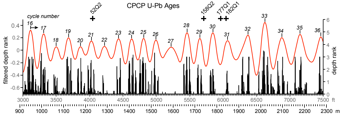
Fig. S7. Filtered depth rank series of NBCP cores overlapping with portion of ages from CPCP13-PFNP-1A core from ref. 16.
