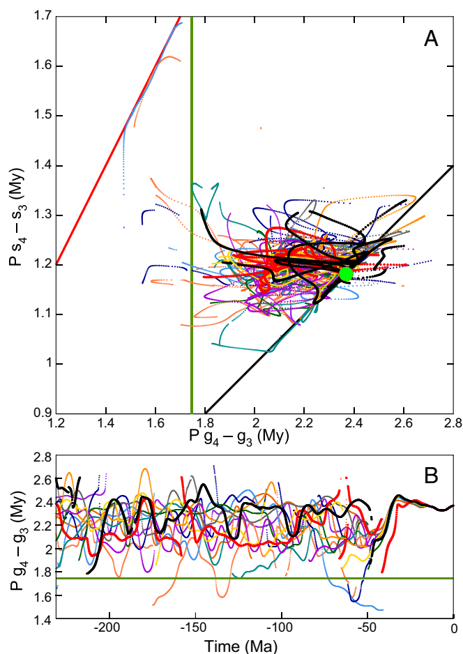
Fig. 7. Evolution of the period (P) of the g_4 - g_3 and s_4 - s_3 terms in 13 numerical solutions of the Solar System integrated over 250 My in the past. Frequencies values are obtained by FA over a sliding interval of 20 My, with an offset of 1 My between each interval. (A) The period of s_4 - s_3 is plotted with respect to the g_4 - g_3 period. The diagonal black line corresponds to the 2:1 resonance [ P(g_4 - g_3) = 2P(s_4 - s_3) ], where P stands for “period of”, while the red line is the 1:1 resonance [ P(g_4 - g_3) = P(s_4 - s_3) ]. The green circle at (2.4, 1.2) is the present value for the Solar System and starting point of all solutions. (B) P(g_4 - g_3) is plotted for all 13 solutions. The black curve corresponds to La2010d (5), and the red curve is the La2004 (29). In both A and B, the green line is P(g_4 - g_3) = 1.75 My, the observed Newark–Hartford value.
