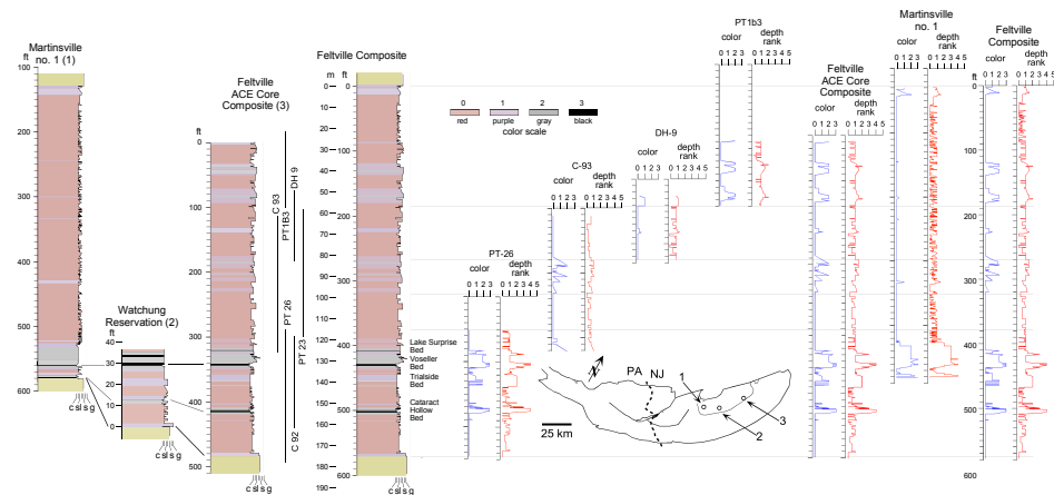
Fig. S3. Construction of the composite Feltville Formation section. Locations are given in Table S1. Note the thinning and onlap of the lower Feltville Formation with the ACE core composite closely approximating the proportions of the correlative lower Shuttle Meadow Formation which has much higher amplitude cyclicity as evidenced in the Silver Ridge core (7).
