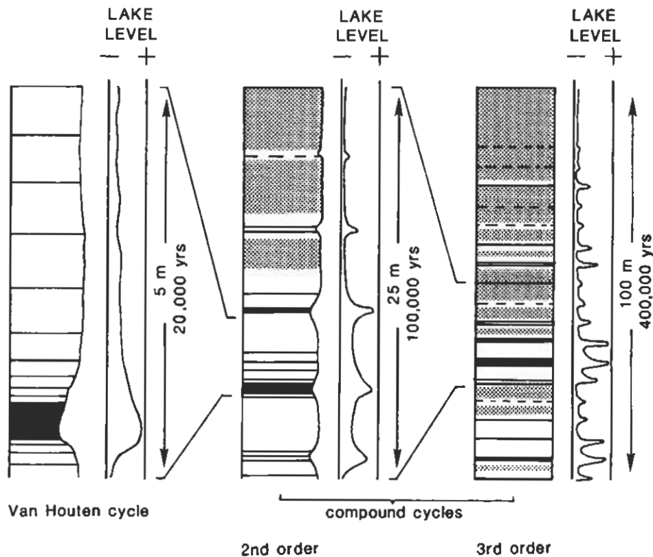
EXPLANATION Black laminated siltstone Gray massive mudstone with desiccation cracks Red massive mudstone with desiccation cracks Figure 4. Idealized Van Houten and compound cycles showing thickness for Lockatong Formation and general interpreted durations and relative lake levels.
