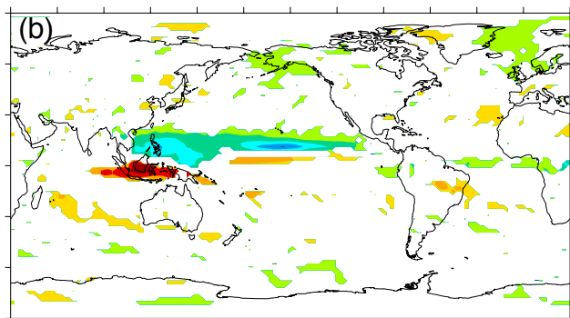
Precipitation change (mm/day)
