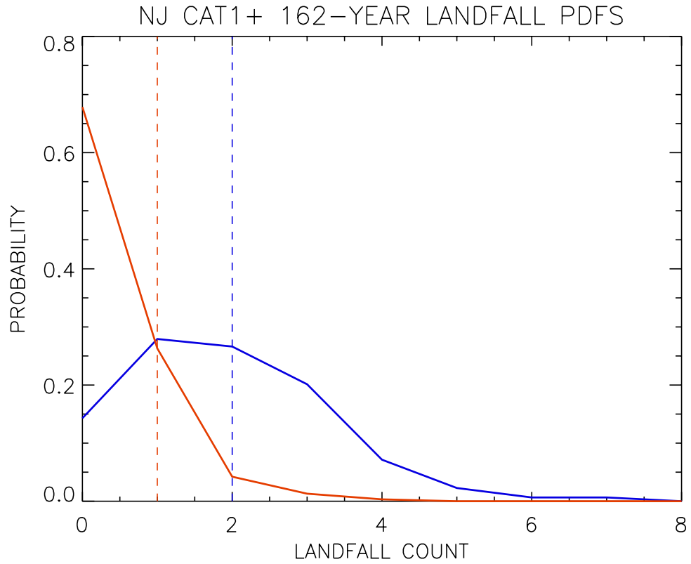
Fig 4: Normalized distributions of NJ CAT1+ landfall counts in 162-year windows from a 50,000-year model simulation. Blue is for all land-falling impact angles, and red is for angles within 30 degrees of perpendicular. The dashed lines at values 2 and 1 indicate the corresponding historical counts that occurred.
