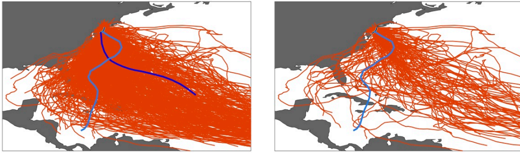
Fig 2: Tropical cyclones (TCs) making landfall on New Jersey. TCs from a 50,000-year neutral climate simulation from the statistical model are shown in red. (a) All TCs making NJ landfall. (b) TCs whose landfalling impact angle is within 30 degrees of perpendicular to the coast segments shown in Fig. 1. The two historical TCs that make NJ landfall in the period 1851-2012 are also shown left: the “Vagabond Hurricane” of Sep., 1903 (dark blue) and Hurricane Sandy (light blue). Only Sandy’s impact angle is within 30 degrees of perpendicular.
