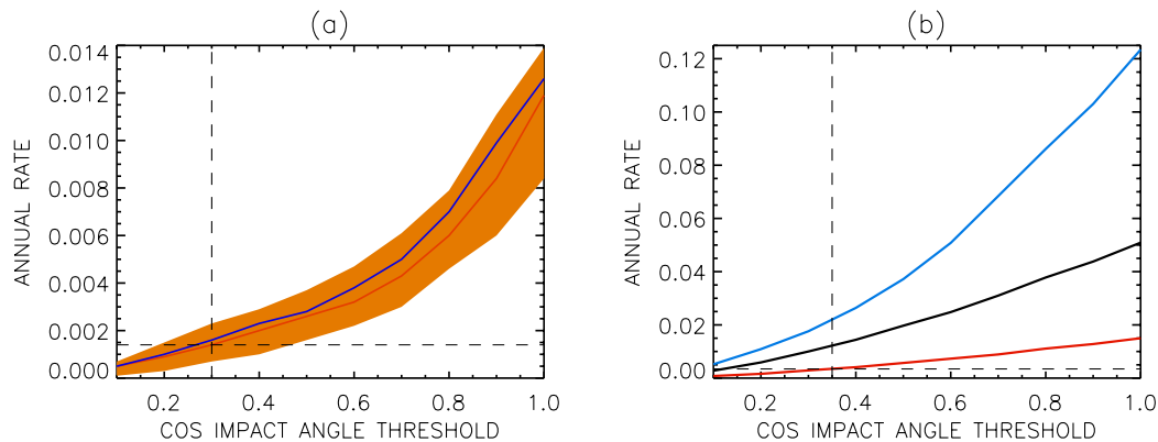
Fig 3: (a) The annual NJ CAT1+ landfall rate as a function of impact angle threshold on the land-falling NJ coast segment. The threshold is expressed as the cos of the angle, \theta , from parallel. Thus, at the right ( \cos(\theta) < 1 or \theta > 0 ) is the rate for all CAT1+
