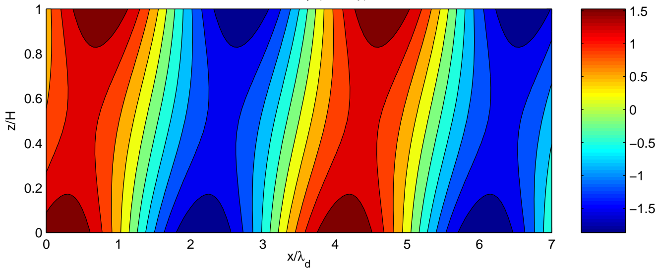
Perturbation \rho (density)
