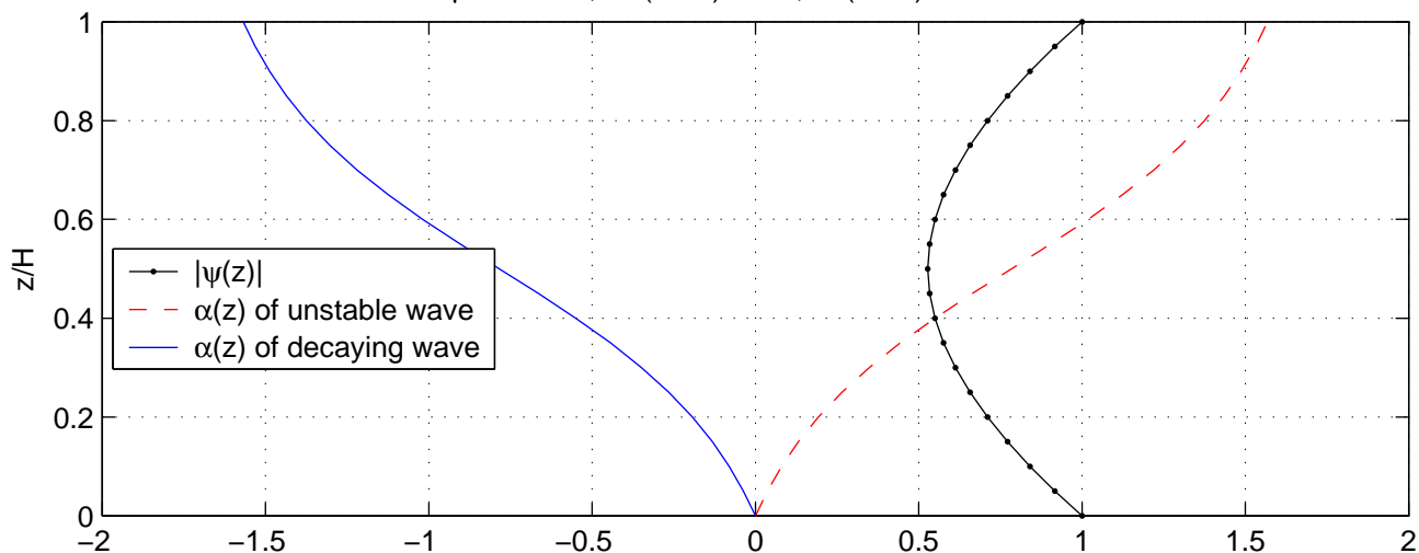
Perturbation \psi (pressure)
