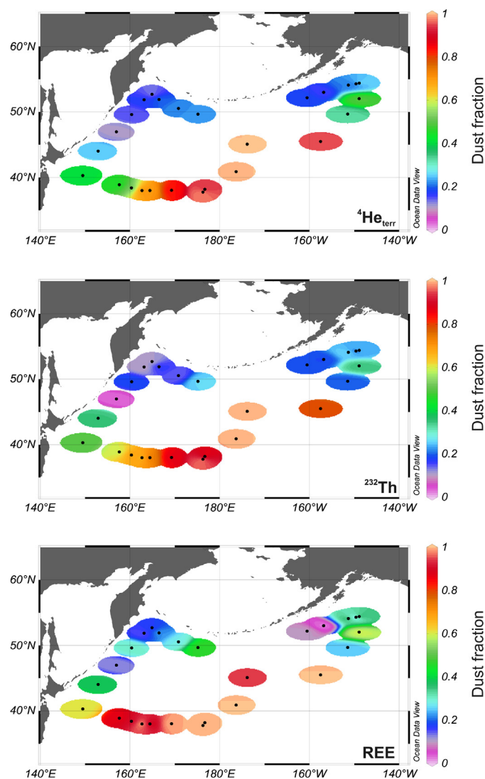
Fig. 5. Dust contributions to the lithogenic fraction for the 26 selected INOPEX multicorer core-top sediment samples shown in Figs. 3 and 4 from the three geochemical tracers ^4\text{He}_{\text{terr}} , ^{232}\text{Th} , and REE. The black dots indicate the locations of the sediment samples. The maps were visualized with a rectangular grid (VG gridding method) with X and Y scale-lengths of 40 and 36°, respectively, using Ocean Data View 4.3.10 (Schlitzer, 2011).
