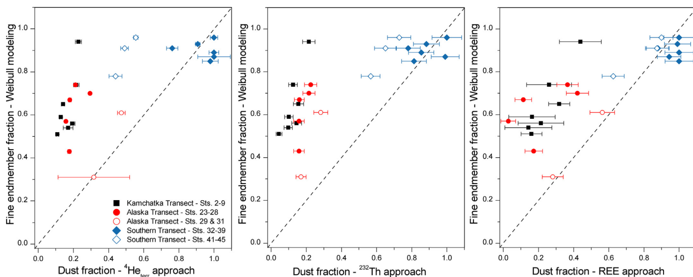
Fig. 6. Comparison of the dust fraction results from the three geochemical tracers ^4\text{He}_{\text{terr}} (left), ^{232}\text{Th} (middle), and REE (right) with the results of the lithogenic fraction of the fine grain size endmember from the Weibull grain size endmember modeling. The black dashed line indicates perfect correlation. The Kamchatka Transect stations 2–9 are shown as black squares, the Alaska Transect stations 23–31 as red circles (stations 29 and 31 as open circles), and the Southern Transect stations 32–45 as blue squares (stations 41, 42, and 45 as open squares). No grain size distribution data are available for stations 1, 26, 37, and 40. (For interpretation of the references to color in this figure legend, the reader is referred to the web version of this article.)
