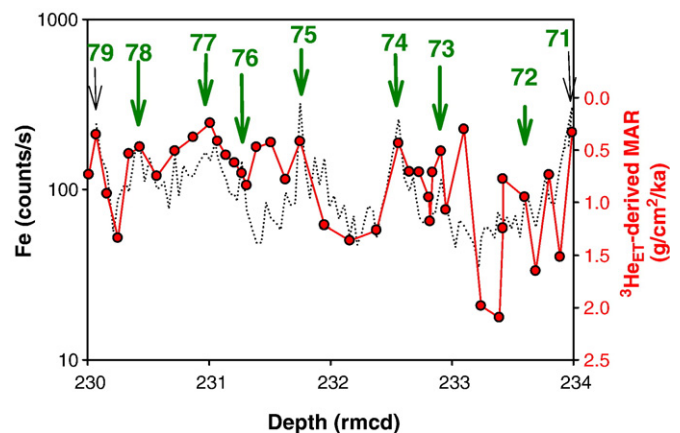
Fig. 4. Depth variations in Fe data and extraterrestrial {}^3\text{He} -derived MARs (reverse scale). The variations in MARs generally follow the 100-kyr eccentricity peaks 71–79 (identified in Fig. 1). Lowest MARs are associated with peaks in eccentricity and vice versa.
