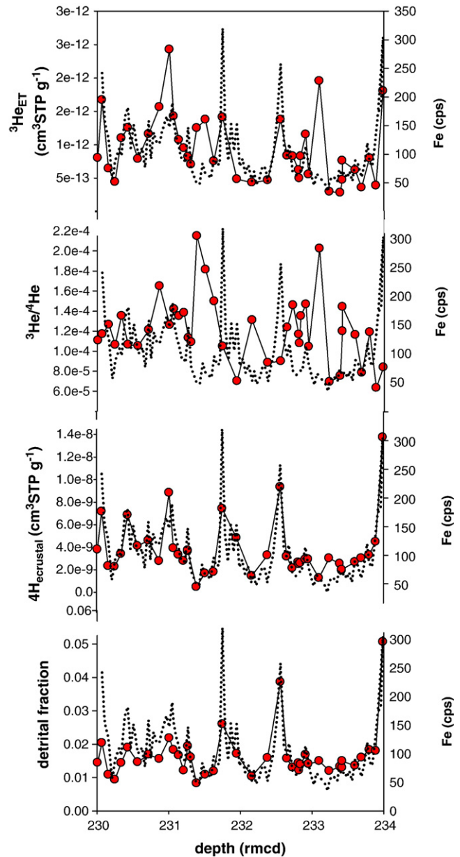
Fig. 2. In each panel the Fe abundance data (XRF counts per second data from Westerhold et al., 2008) is plotted against revised meters composite depth (rmcd), along with a) extraterrestrial ^3\text{He} content, b) ^3\text{He}/^4\text{He} isotope ratio, c) ^4\text{He}_{\text{crustal}} (terrestrially-derived ^4\text{He} ) content, and d) detrital fraction (assumed to be the non-dissolvable fraction of the sediment).
