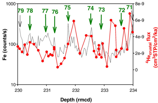
Fig. 5. Depth variations in the flux of ^4\text{He}_{\text{crustal}} derived using the ^3\text{He} -calculated MARs. The flux of ^4\text{He}_{\text{crustal}} is an estimate of the flux of windblown dust from the continents. For the most part, highest ^4\text{He}_{\text{crustal}} fluxes coincide with peaks in eccentricity.
