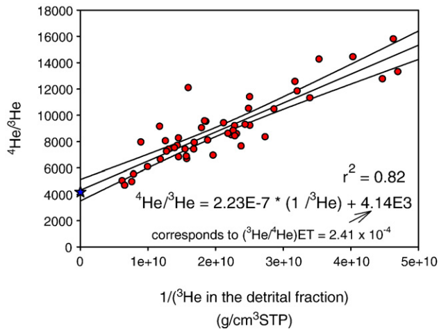
Fig. 3. ^4\text{He}/^3\text{He} isotope ratio plotted against 1/{}^3\text{He} (non-dissolvable). The data are linearly correlated ( r^2=0.82 ; 1\sigma error regression envelope drawn around line). The intercept approximates the ^4\text{He}/^3\text{He} isotope ratio of the extraterrestrial IDP end-member. The blue star is the average helium isotope ratio and {}^3\text{He} concentration values for modern-day IDPs measured by Nier and Schlutter (1992).
